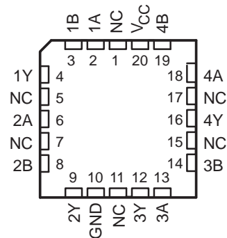
SN54AS1032A . . . FK PACKAGE (TOP VIEW)
