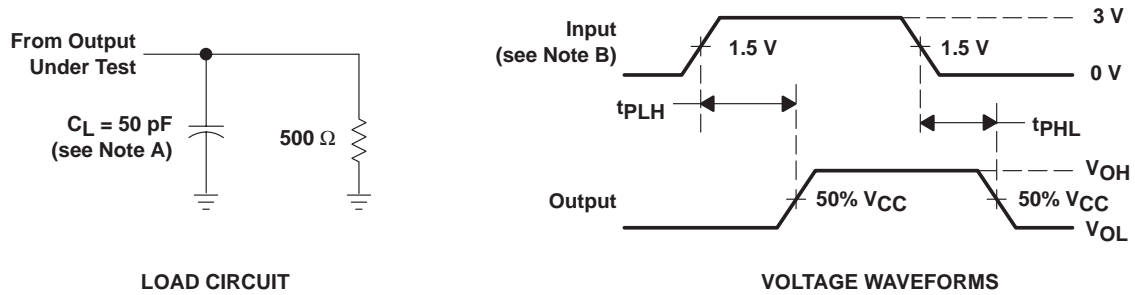
LOAD CIRCUIT
