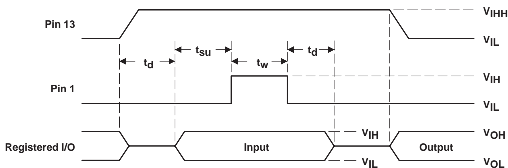
Figure 1. Preload Waveforms
