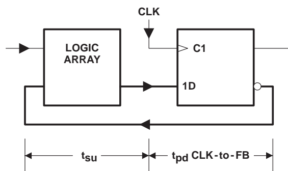
Figure 4. f_{\max} With Internal Feedback
