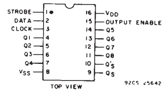
Fig. 1 – Terminal assignment.
