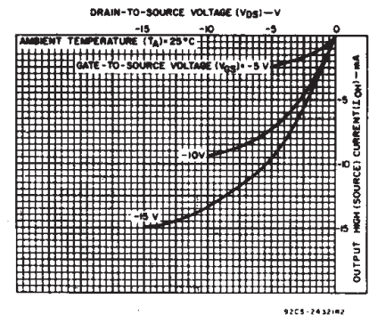
Fig. 7 — Minimum output high (source) current characteristics.
