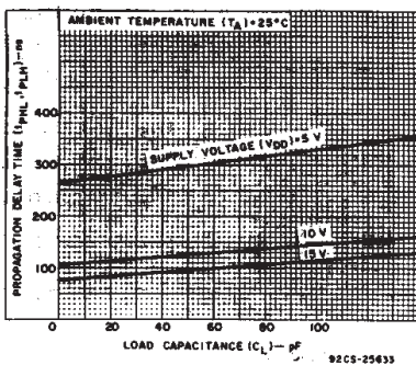
Fig. 8 — Clock-to-serial output Q_S propagation delay vs C_L .
