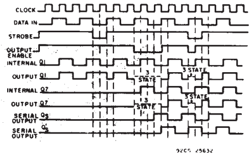
Fig. 3 – Timing diagram.
