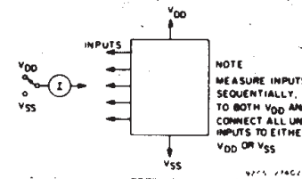
Fig. 19 - Input current test circuit.
