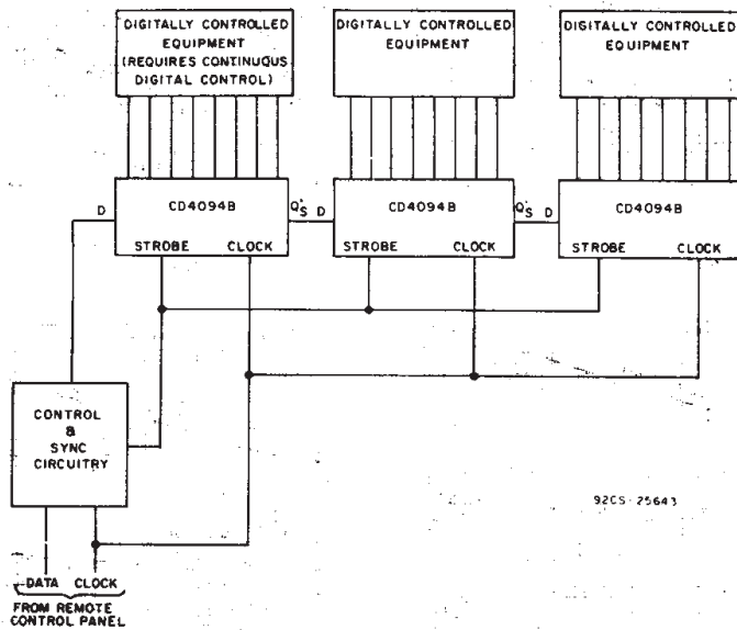
Fig. 14 - Remote control holding register.
