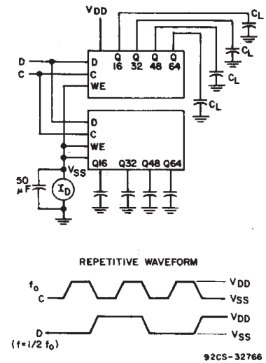
Fig. 11—Dynamic power dissipation test circuit and waveforms.
