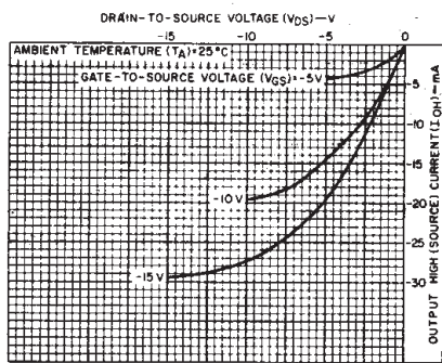
Fig. 6—Typical p-channel output high (source) current characteristics.
