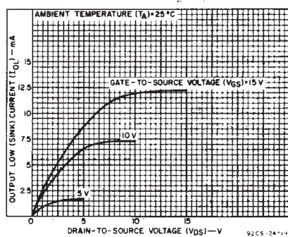
Fig. 5—Minimum n-channel output low (sink) current characteristics.
