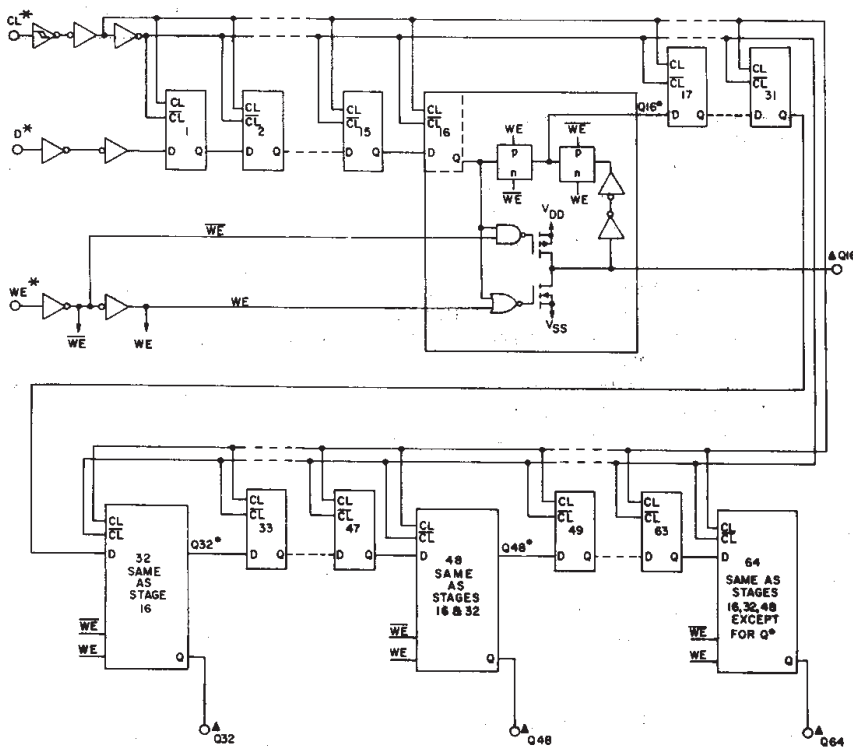
Fig. 1—CD4517B functional block diagram (one half).
