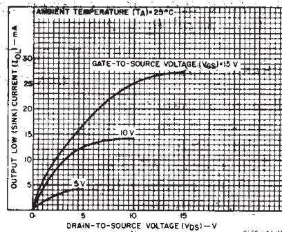
Fig. 4—Typical n-channel output low (sink) current characteristics.
