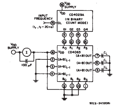
Fig. 12 - Dynamic power dissipation test circuit.
