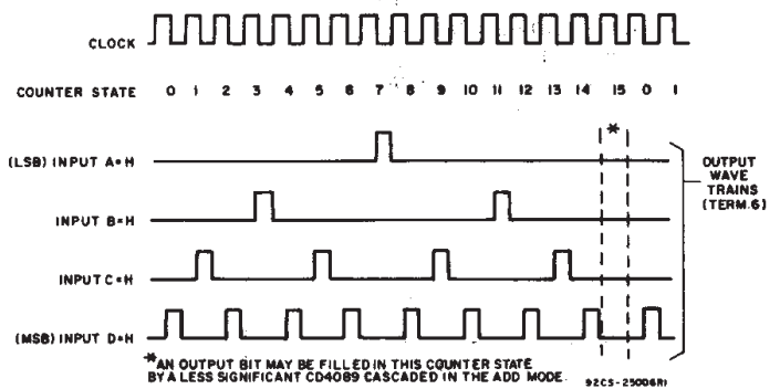
Fig. 15 - Timing diagram.
