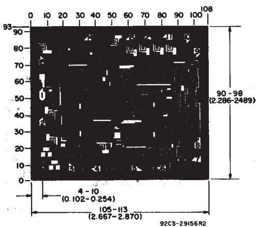
Dimensions and Pad Layout for CD4089BH
