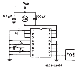
Fig. 9 — Dynamic power dissipation test circuit.
