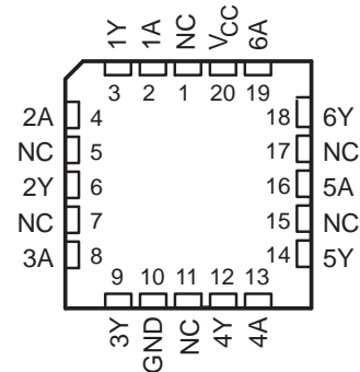
SN54ALS1035 . . . FK PACKAGE (TOP VIEW)
