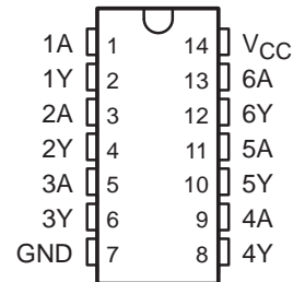
SN54ALS1035 . . . J PACKAGE SN74ALS1035 . . . D OR N PACKAGE (TOP VIEW)
