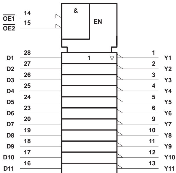
logic symbol†
