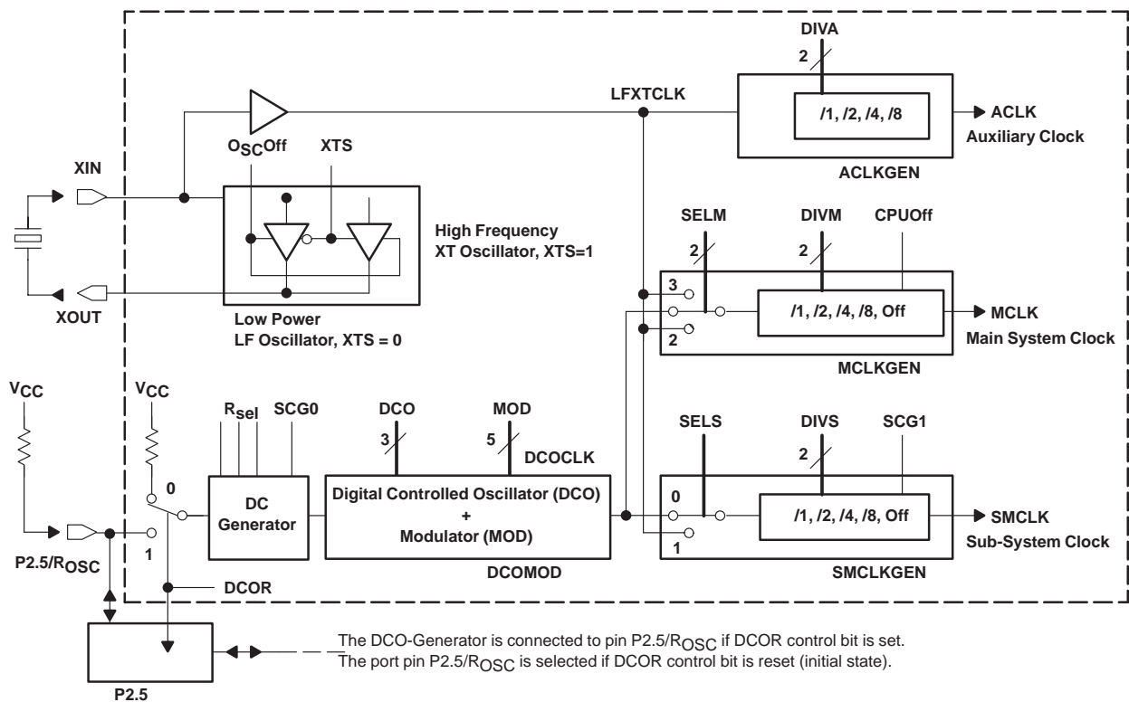
Figure 1. Clock Signals
