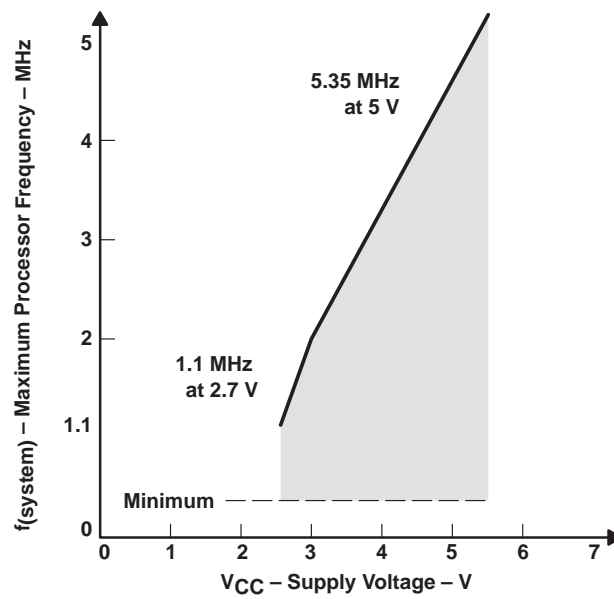
Figure 4. P/E Version Frequency vs Supply Voltage
