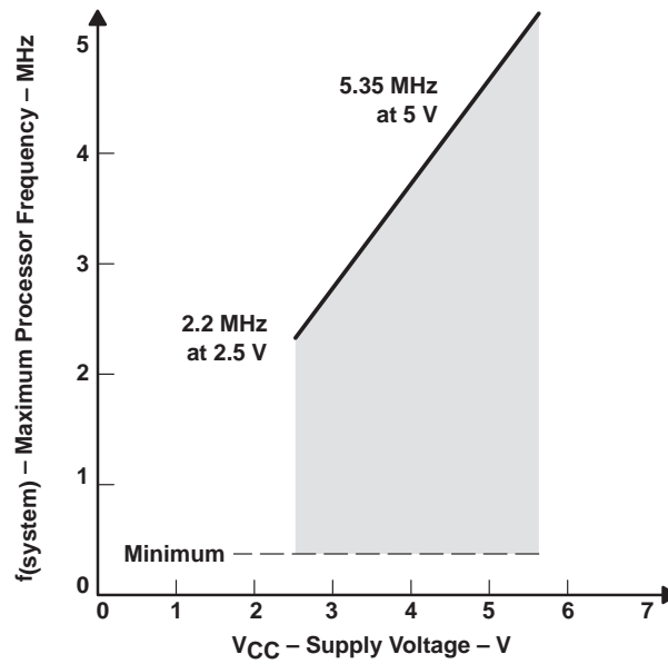
Figure 3. C Version Frequency vs Supply Voltage
