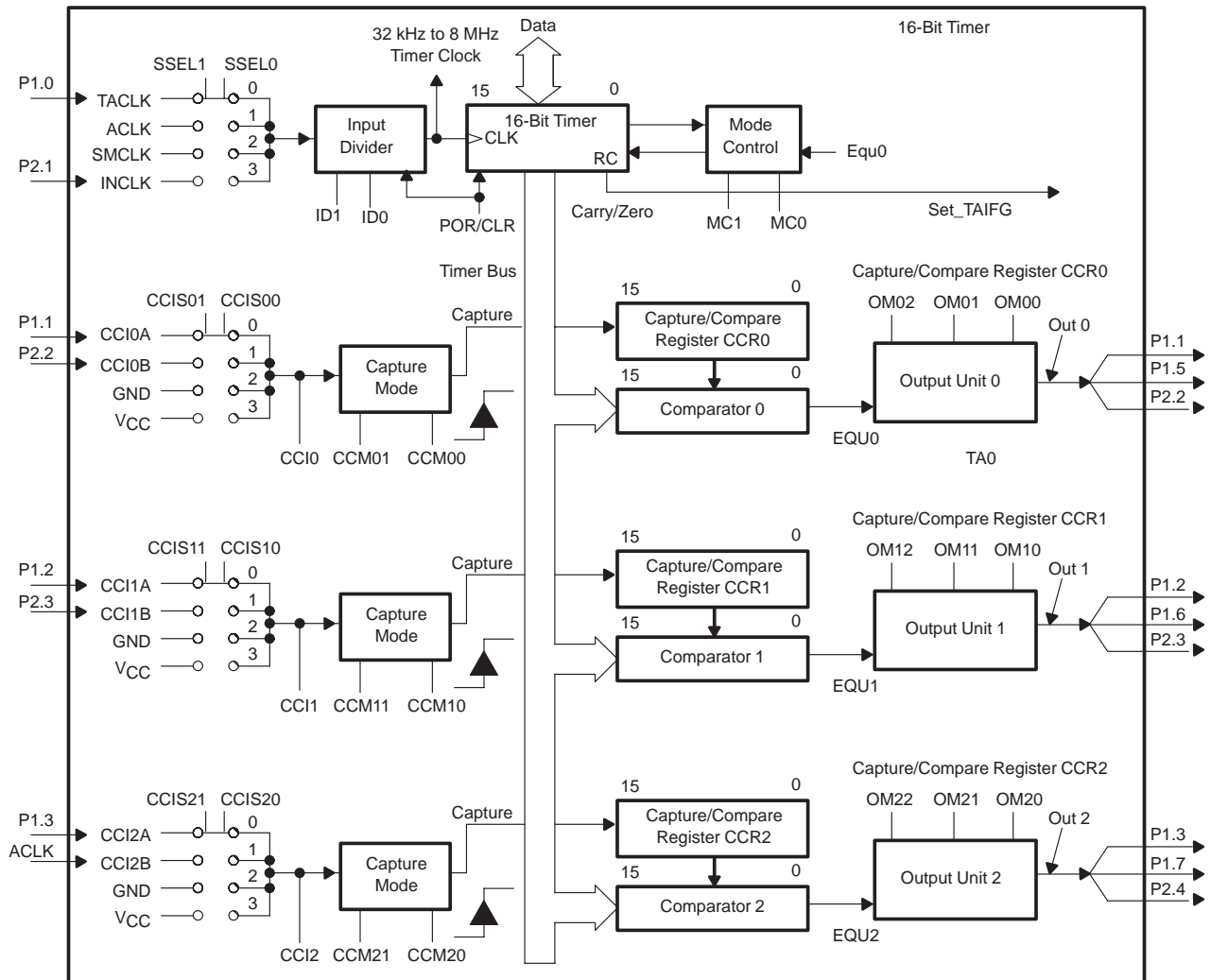
Figure 2. Timer_A, MSP430x11x Configuration
