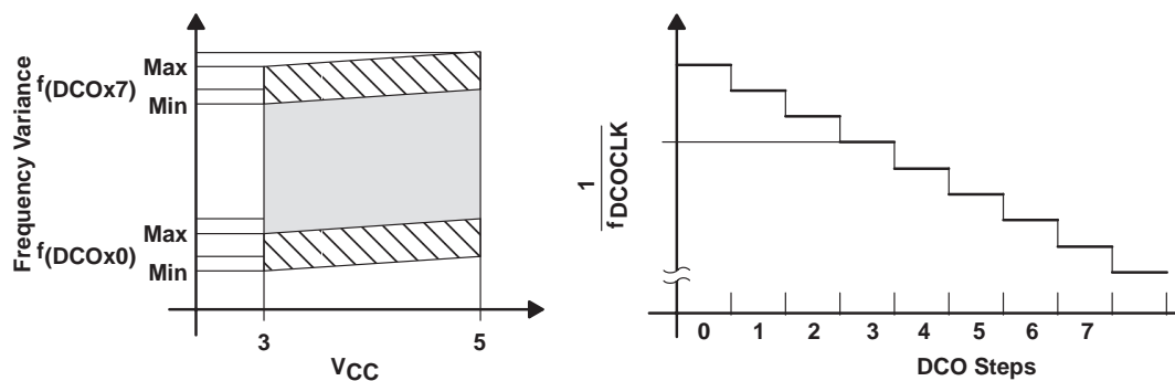
Figure 7. DCO Characteristics
