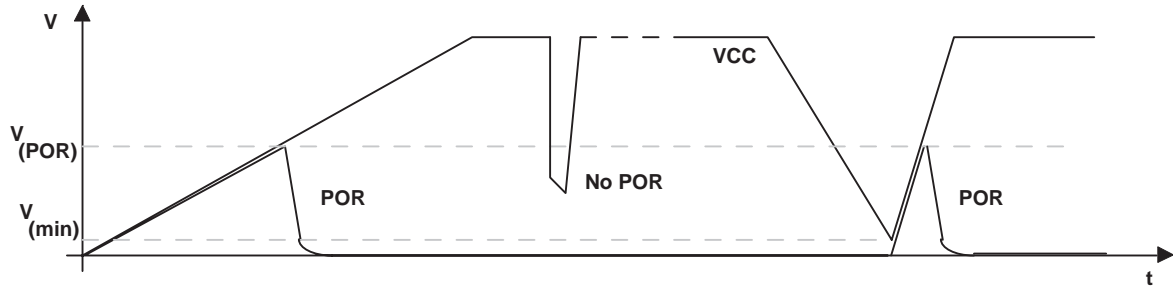
Figure 5. Power-On Reset (POR) vs Supply Voltage
