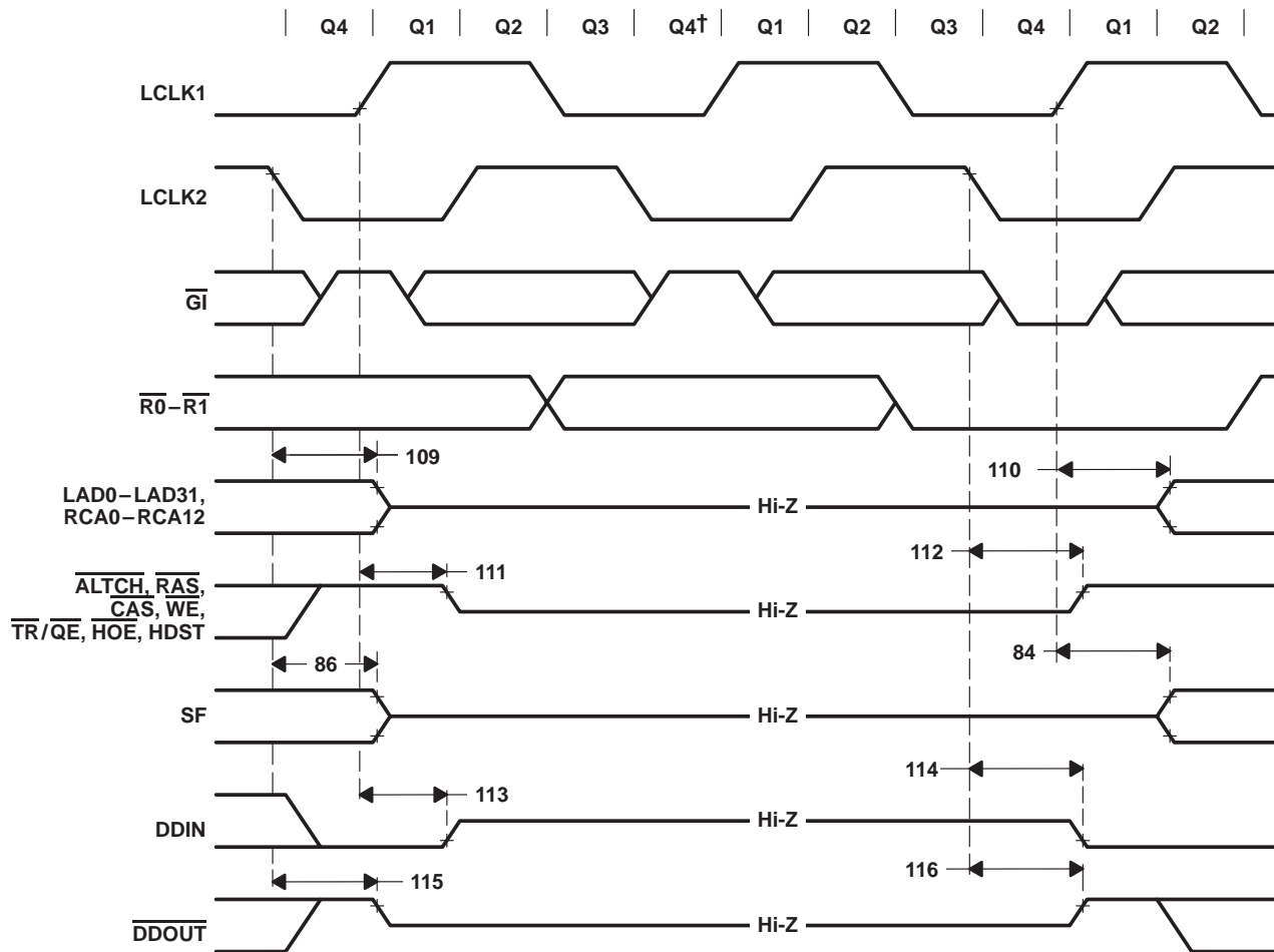
Figure 45. Multiprocessor-Interface Timing: High-Impedance Signals
