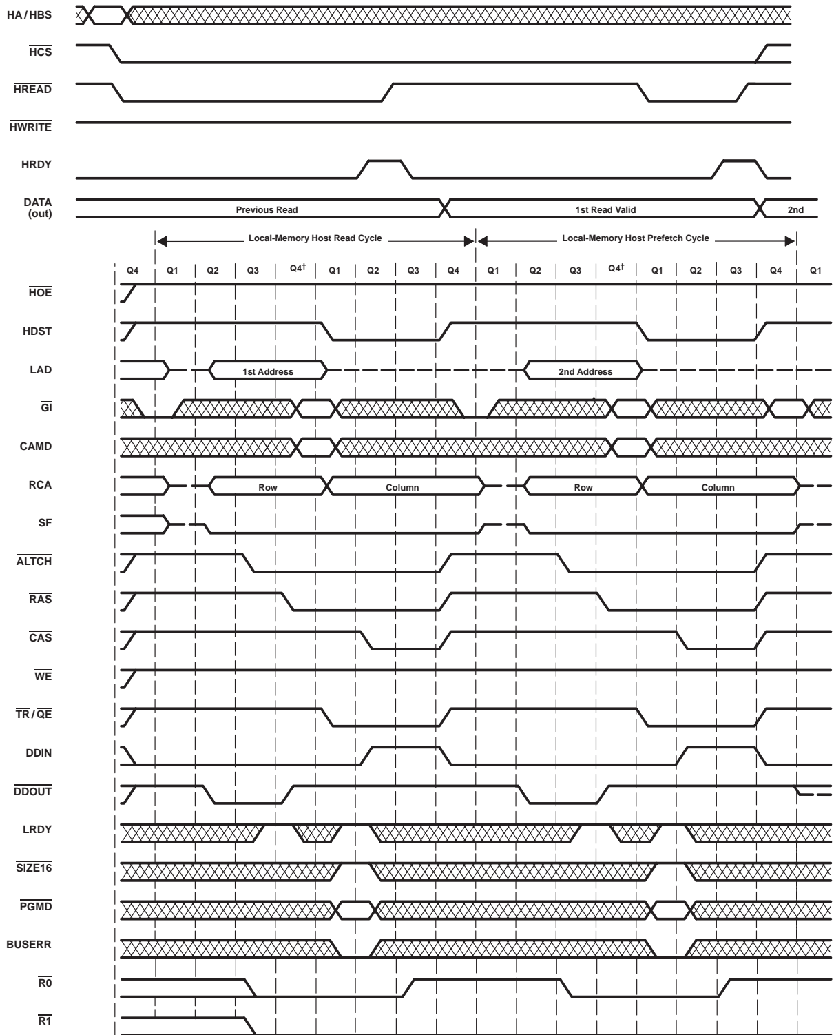
Figure 21. Back-to-Back Host-Read Cycles With Implicit Addressing; HREAD as Strobe
