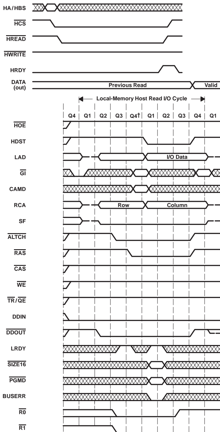
Figure 22. Host-Read Cycle Timing From SMJ34020A I/O Registers
