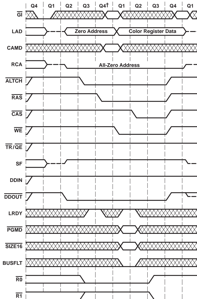
Figure 10. Load-Color-Latch-Cycle Timing
