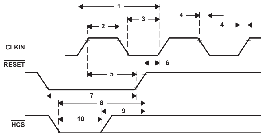
Figure 33. CLKIN and \overline{\text{RESET}} Timing Requirements
