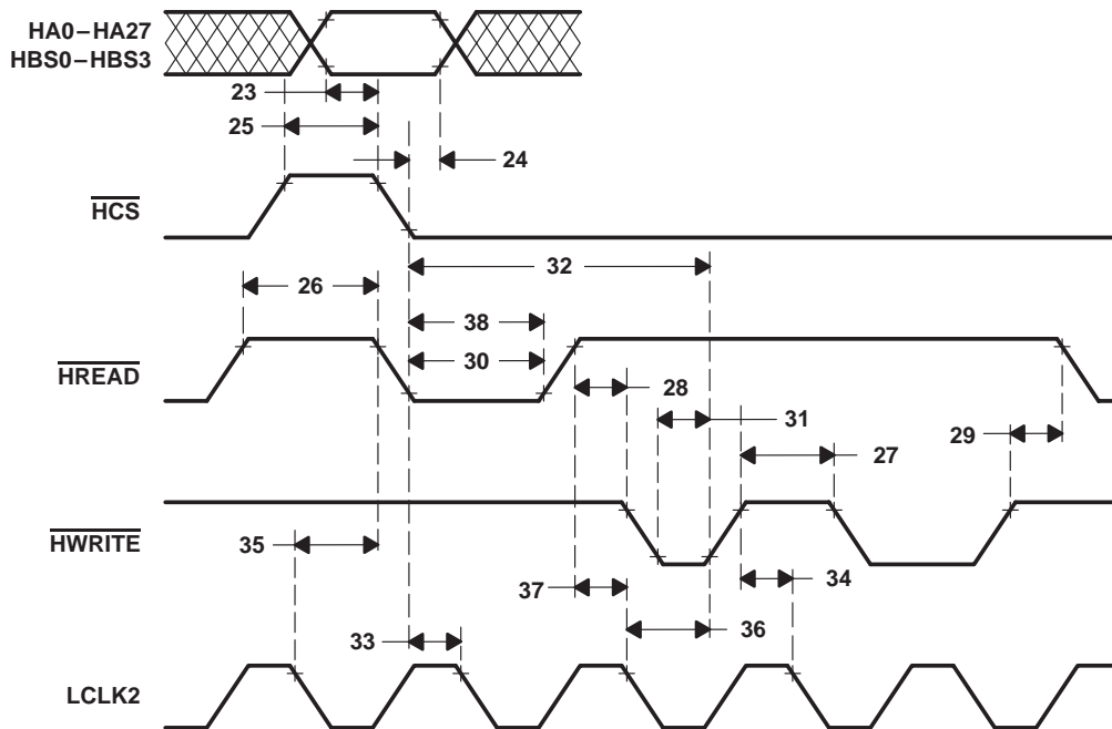
Figure 36. Host-Interface-Cycle Timing Requirements
