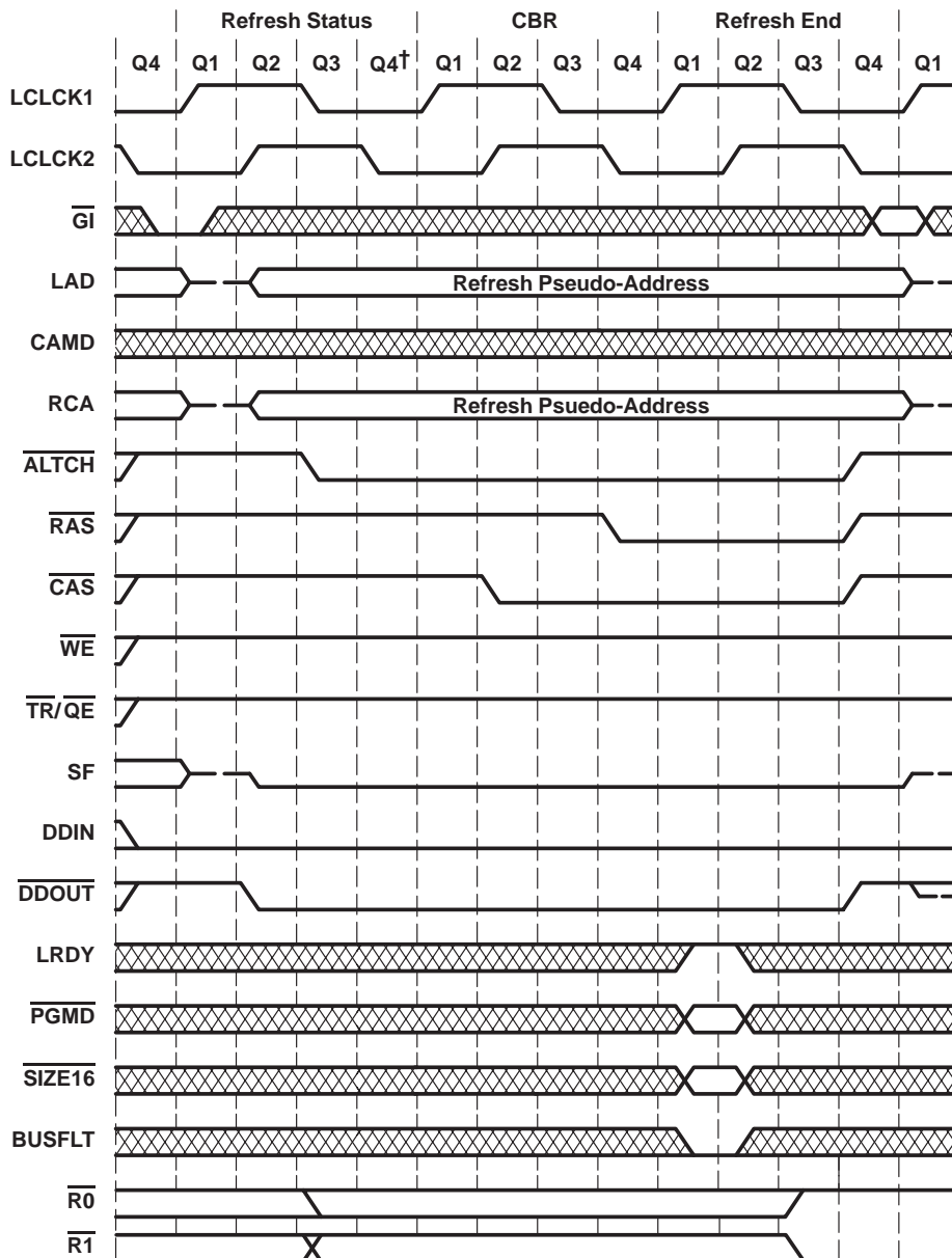
Figure 6. Refresh-Cycle Timing
