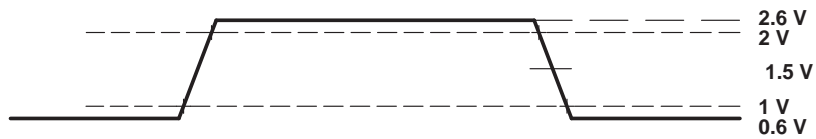
Figure 31. TTL-Level Outputs
