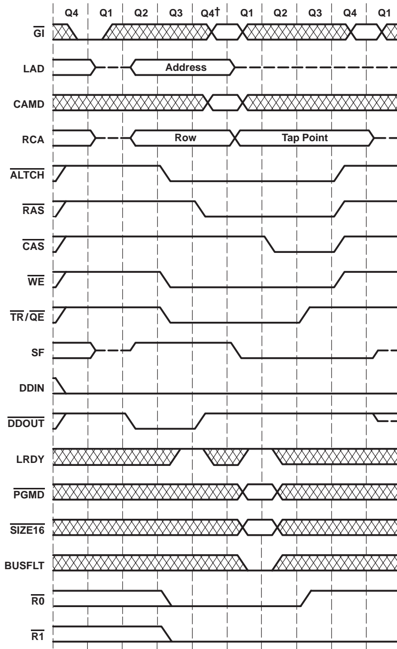
Figure 17. Serial-Data-Register-to-Memory Cycle Timing (VRAM-Alternate-Write Transfer)
