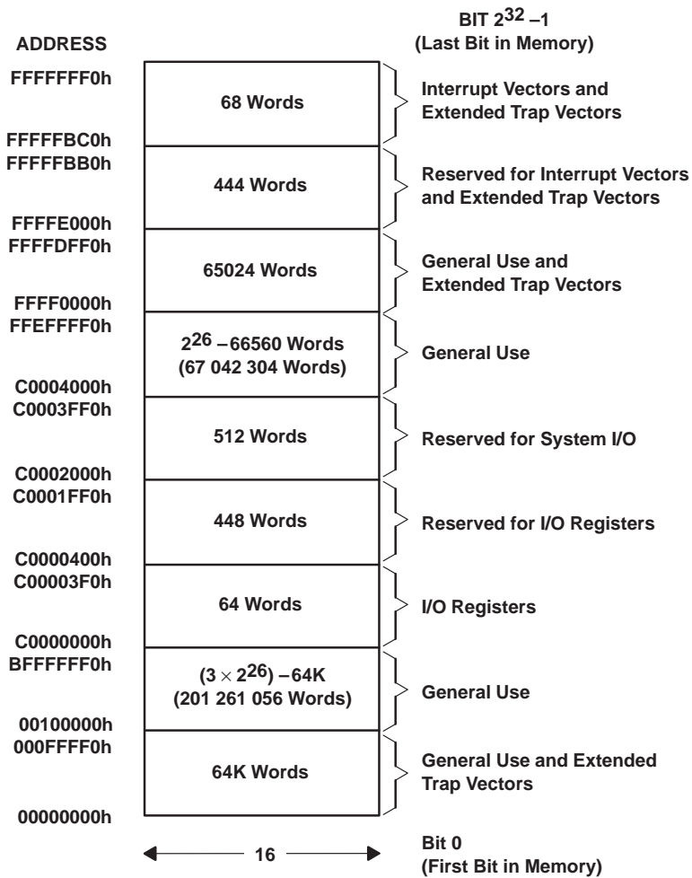
Figure 1. Memory Map
