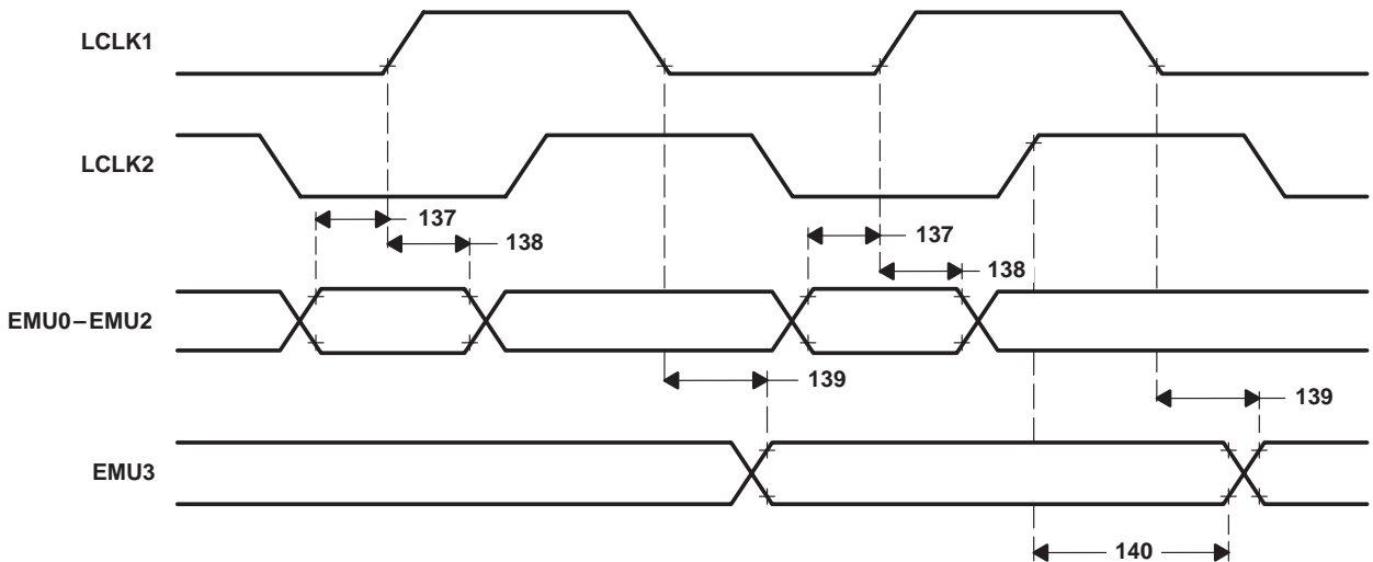
Figure 51. Emulator-Interface Timing
