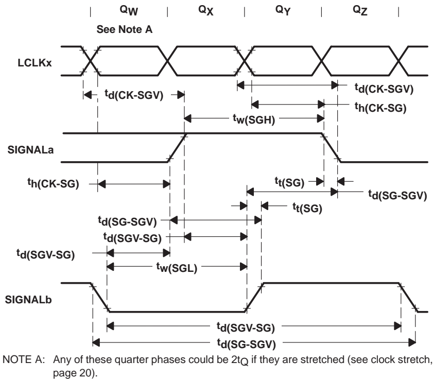
Figure 35. Output Signal Characteristics
