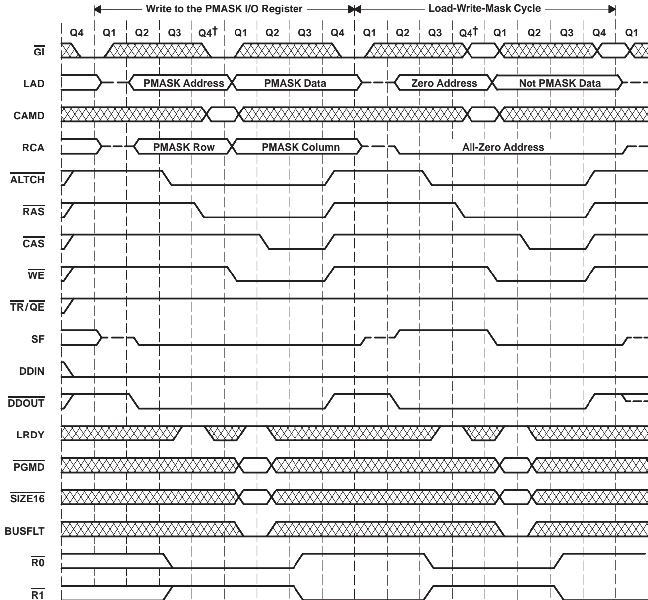
Figure 9. Load-Write-Mask-Cycle Timing
