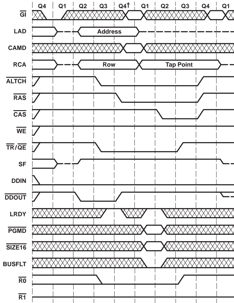
Figure 15. Memory-to-Split-Serial-Data-Register-Cycle Timing (VRAM Split-Register Read Transfer)
