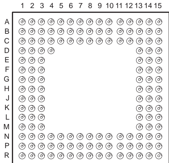
145-PIN GRID ARRAY PACKAGE (BOTTOM VIEW)
