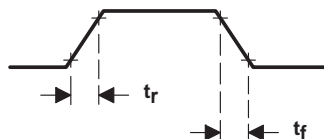
Figure 26. Signal-Switching Timing
