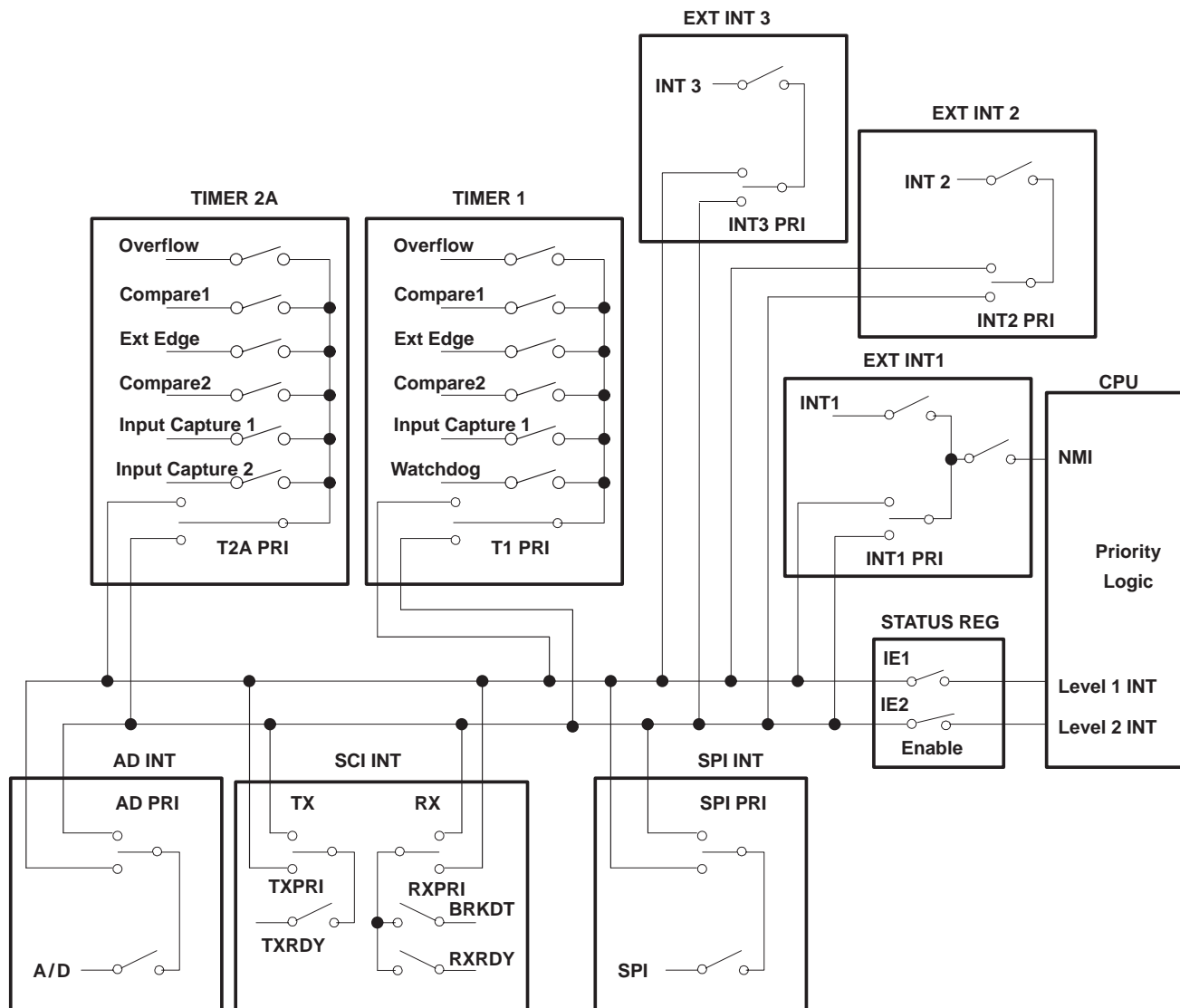
Figure 4. Interrupt Control
