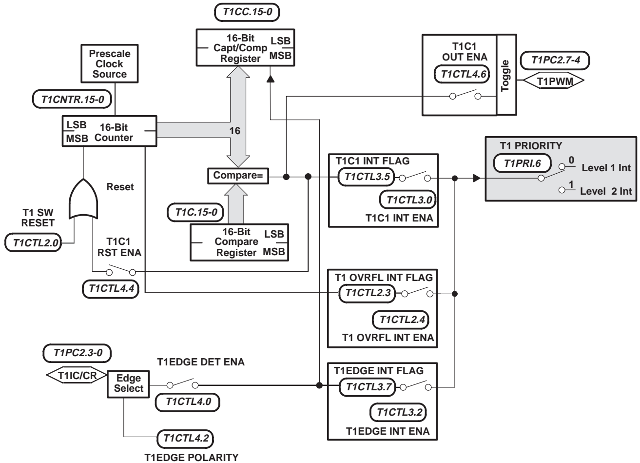
Figure 6. Capture/Compare Mode
