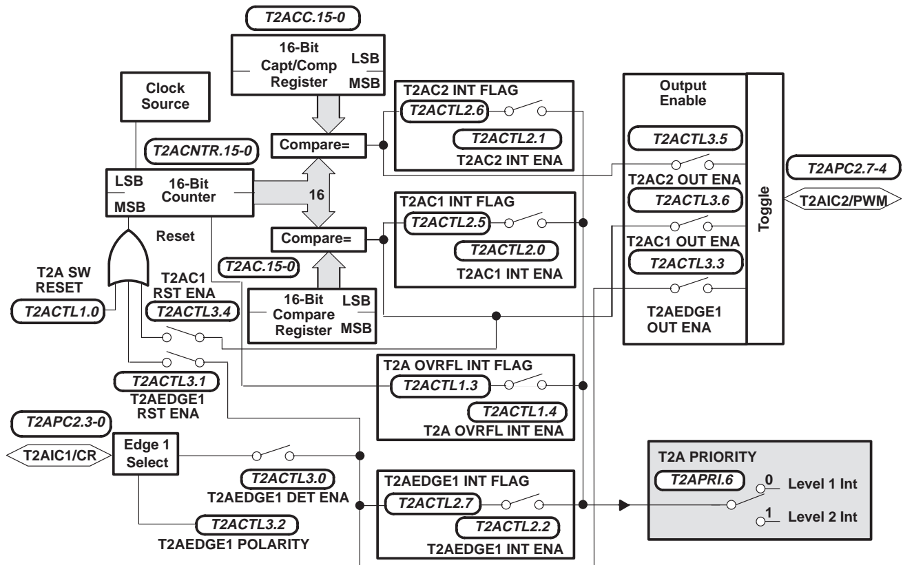
Figure 12. Dual-Compare Mode
