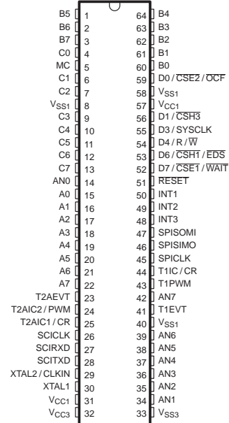
JN/NM PACKAGE (TOP VIEW)
