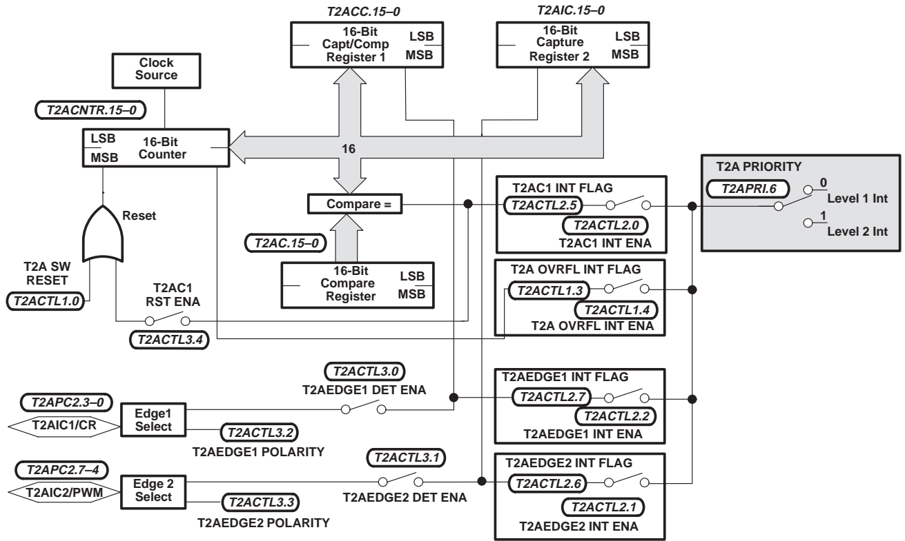
Figure 13. Dual-Capture Mode
