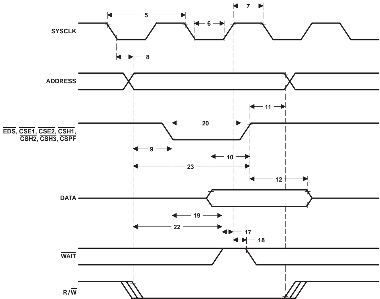
Figure 28. Switching Characteristics and Timing Requirements for External-Write
