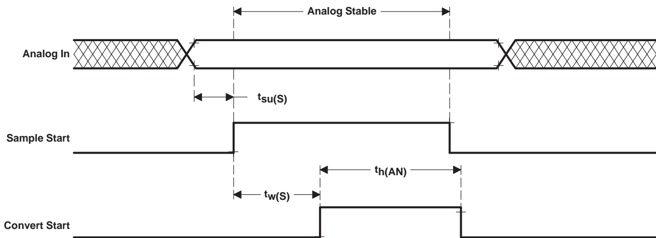
Figure 33. Analog Timing
