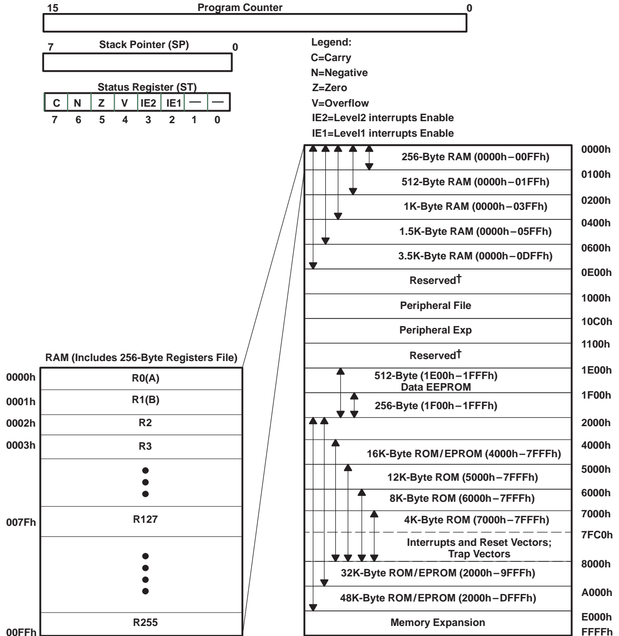
Figure 1. Programmer's Model
