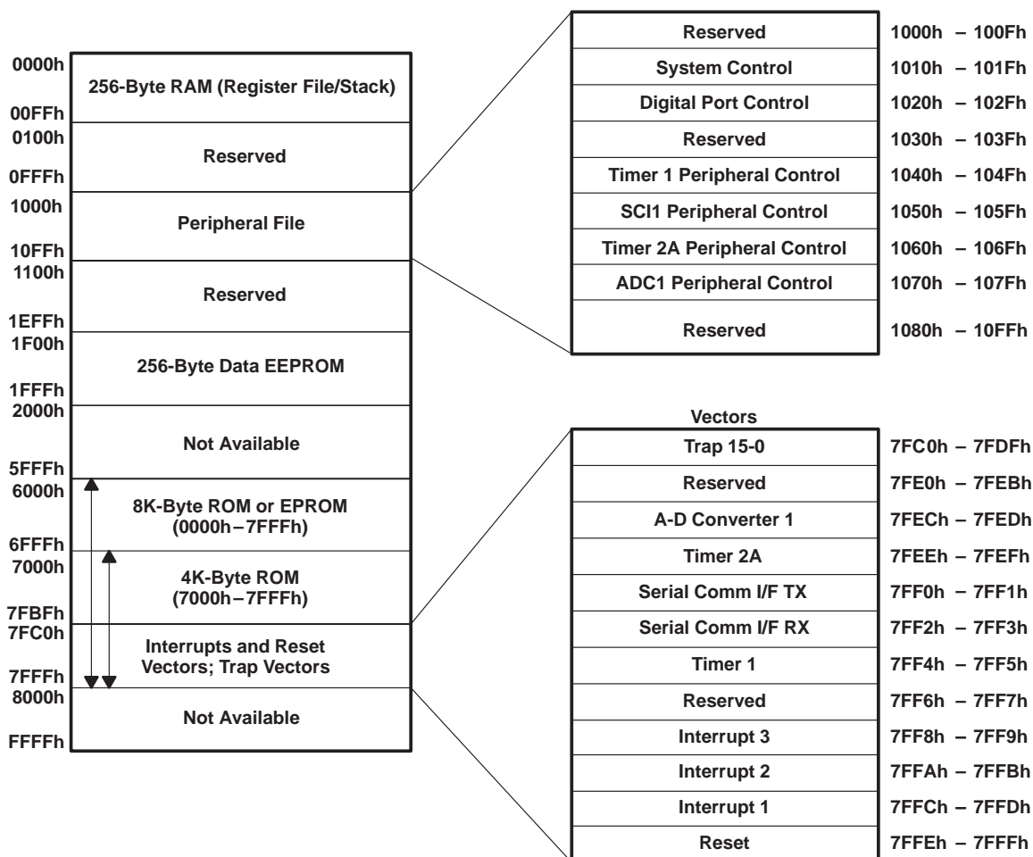
Figure 3. TMS370Cx4x Memory Map
