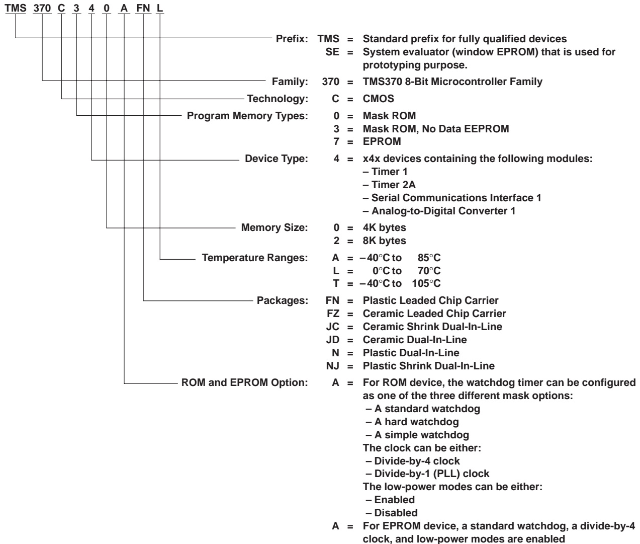
Figure 16. TMS370Cx4x Family Nomenclature
