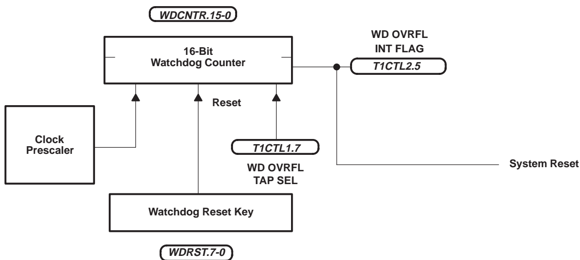
Figure 9. Hard Watchdog
