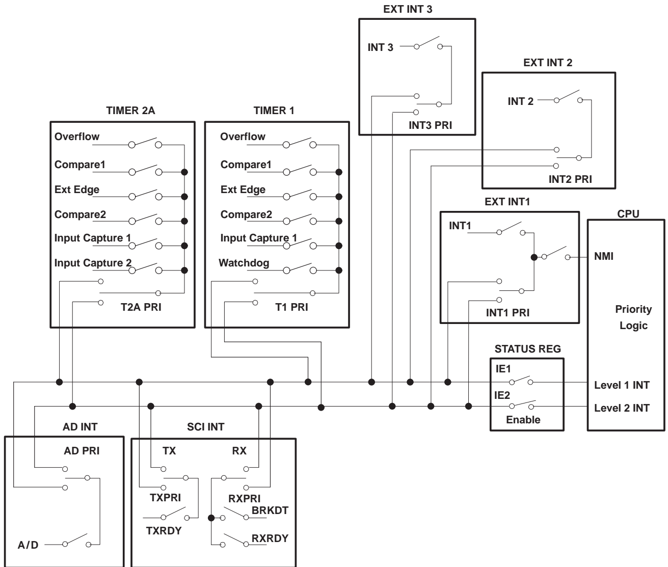
Figure 4. Interrupt Control
