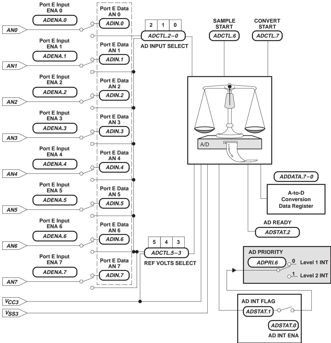
Figure 15. ADC1 Converter Block Diagram
