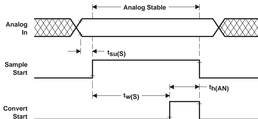
Figure 23. Analog Timing
