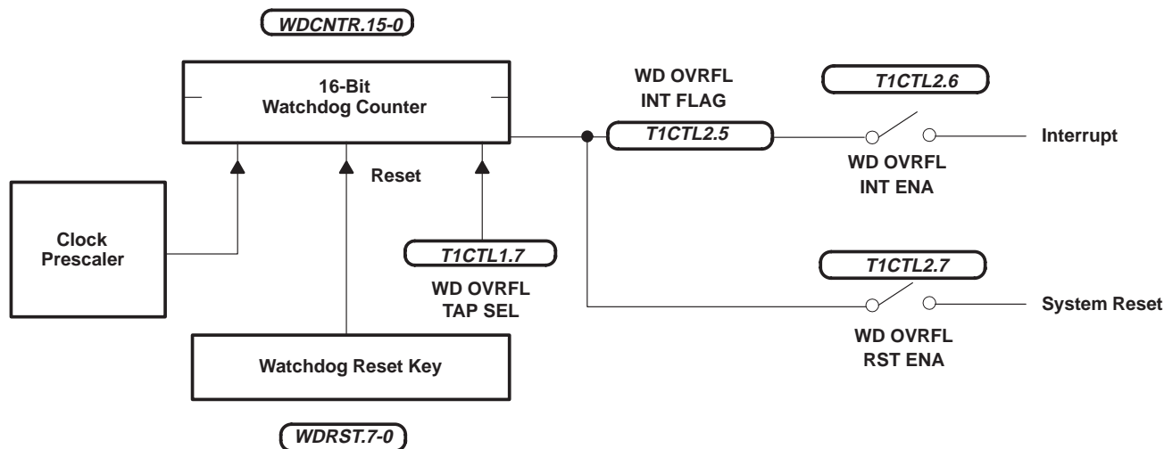
Figure 8. Standard Watchdog
