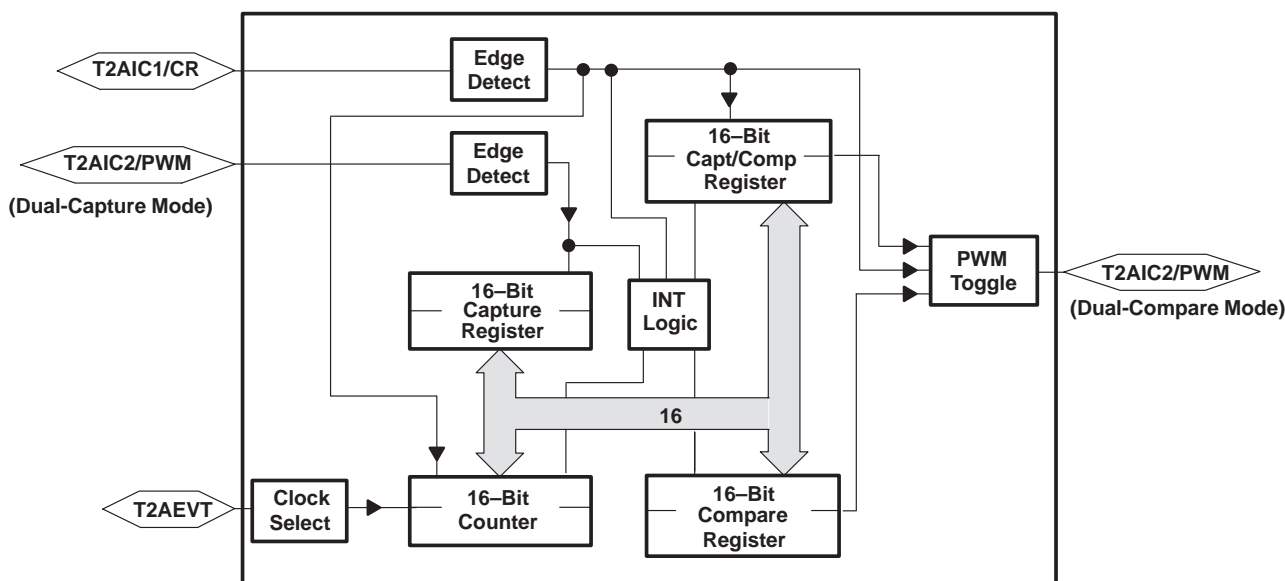
Figure 11. Timer 2A Module Block Diagram
