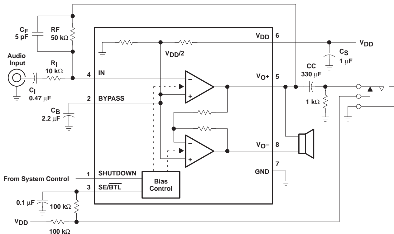
Figure 51. TPA711 Application Circuit
