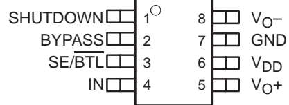
D OR DGN PACKAGE (TOP VIEW)
