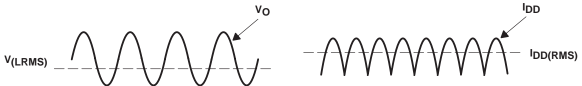
Figure 36. Voltage and Current Waveforms for BTL Amplifiers
