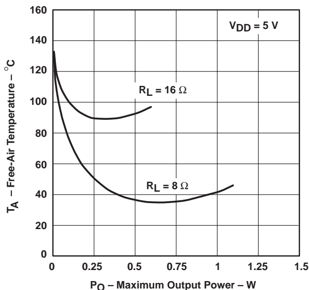
Figure 39. Free-Air Temperature vs Maximum Continuous Output Power
