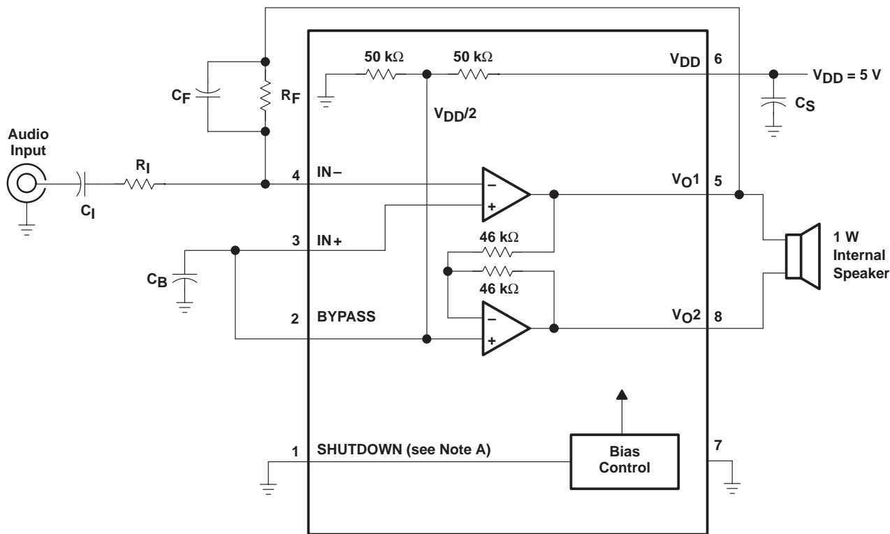
Figure 37. TPA4861 Typical Notebook Computer Application Circuit
