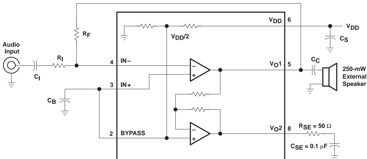
Figure 38. Singled-Ended Mode
