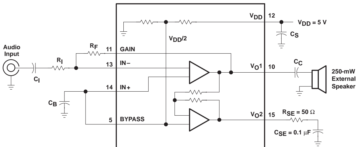
Figure 38. Singled-Ended Mode
