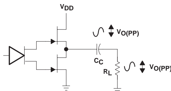
Figure 35. Single-Ended Configuration
