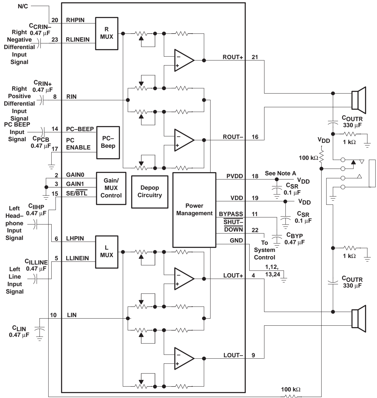
Figure 43. Typical TPA0112 Application Circuit Using Differential Inputs
