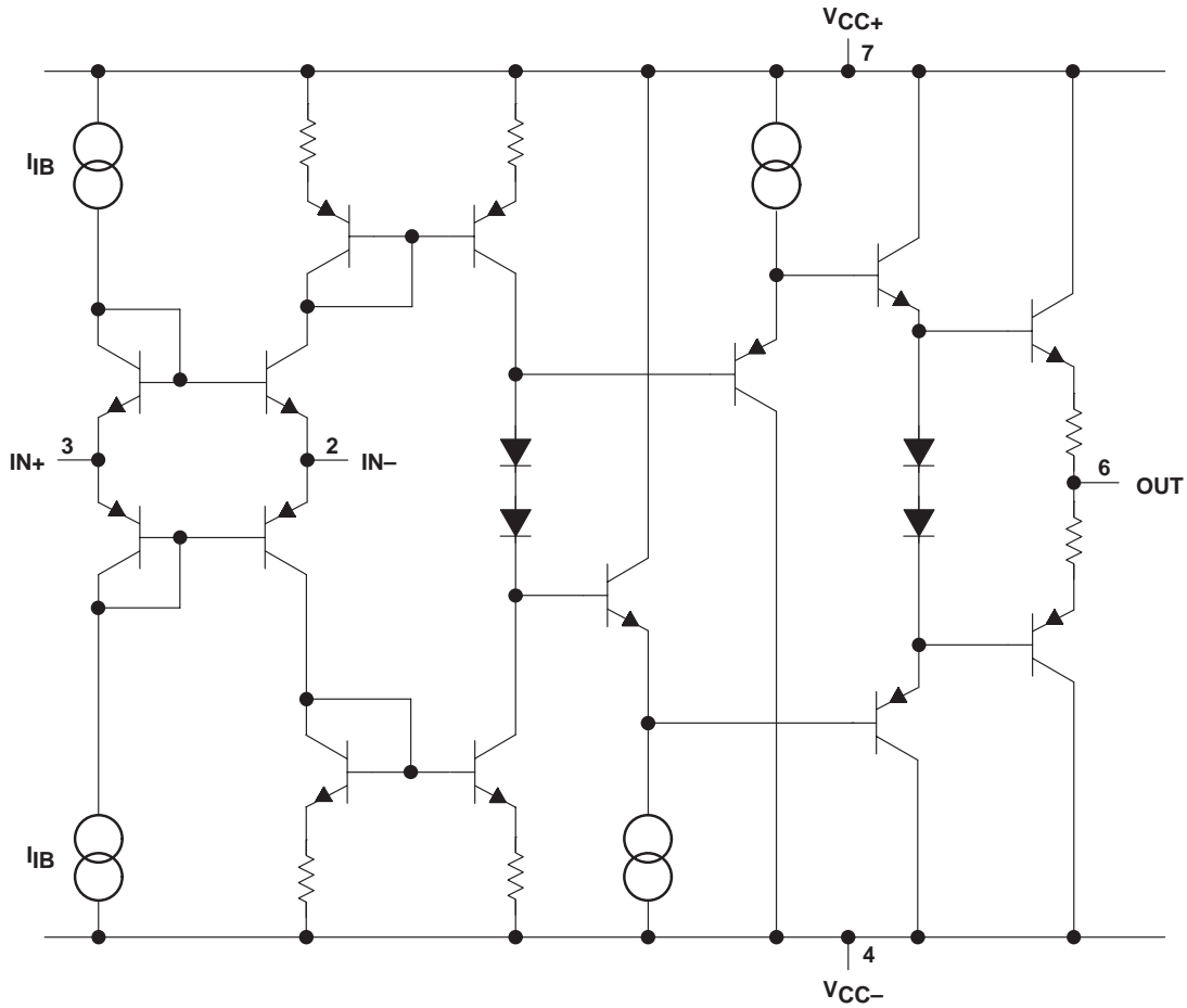
Figure 47. Simplified Schematic
