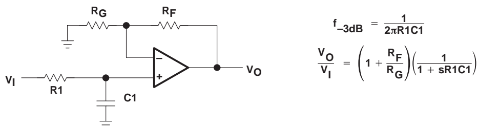
Figure 57. Single-Pole Low-Pass Filter
