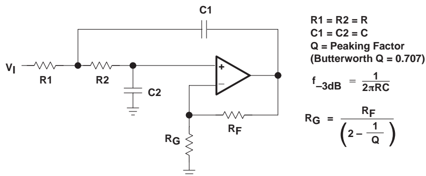
Figure 58. 2-Pole Low-Pass Sallen-Key Filter
