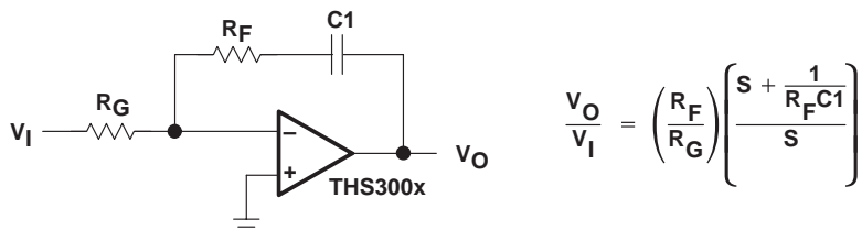
Figure 59. Inverting CFB Integrator
