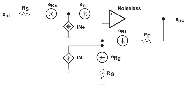
Figure 49. Noise Model
