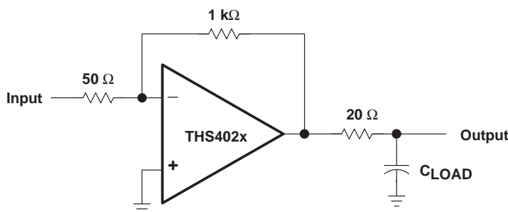
Figure 33. Driving a Capacitive Load
