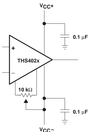
Figure 34. Offset Nulling Schematic
