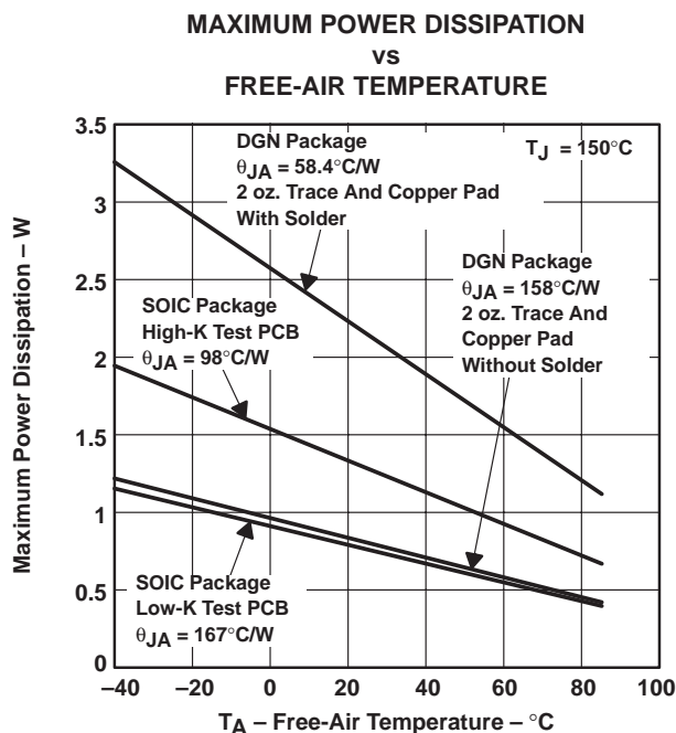
Figure 39. Maximum Power Dissipation vs Free-Air Temperature
