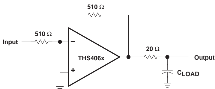
Figure 25. Driving a Capacitive Load
