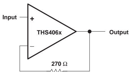
Figure 24. Noninverting, Unity Gain Schematic
