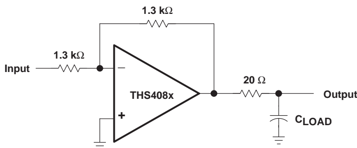
Figure 41. Driving a Capacitive Load
