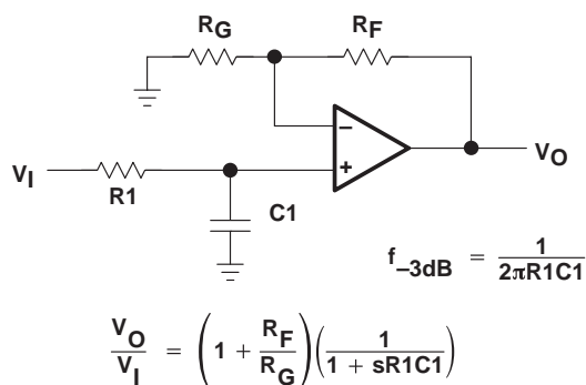
Figure 43. Single-Pole Low-Pass Filter
