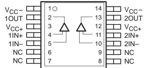
Thermally Enhanced TSSOP (PWP) PowerPAD™ Package (TOP VIEW)
