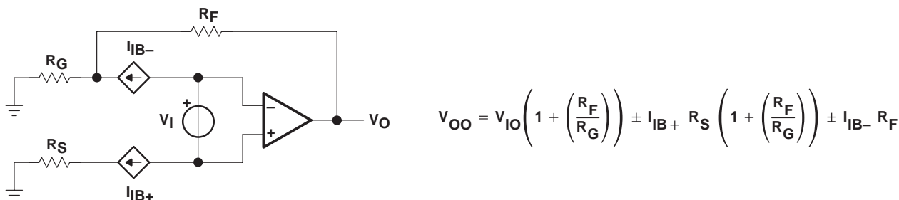
Figure 50. Output Offset Voltage Model
