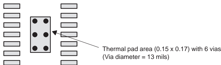
Figure 58. PowerPAD PCB Etch and Via Pattern – Minimum Requirements
