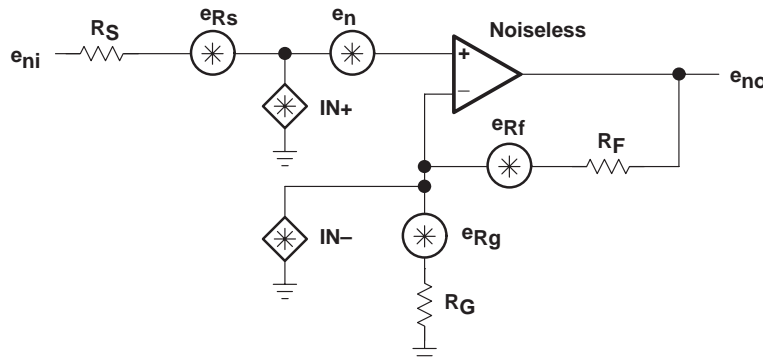
Figure 51. Noise Model
