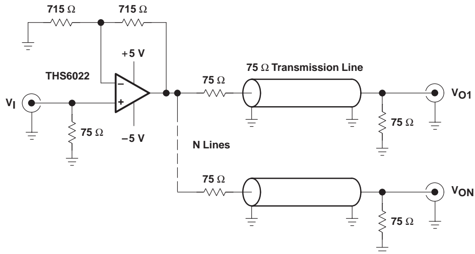
Figure 65. Video Distribution Amplifier Application
