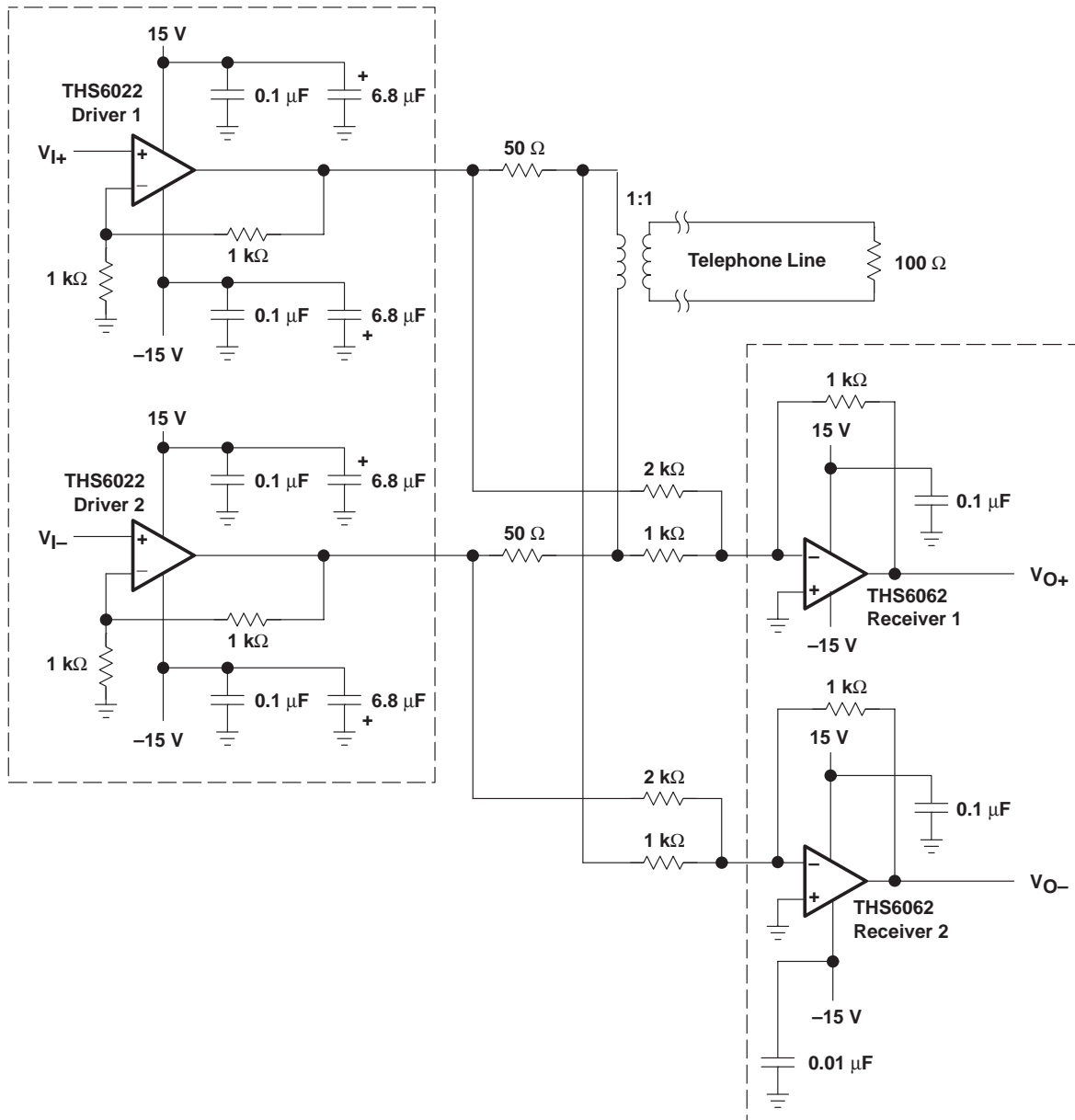
Figure 60. THS6022 ADSL Application
