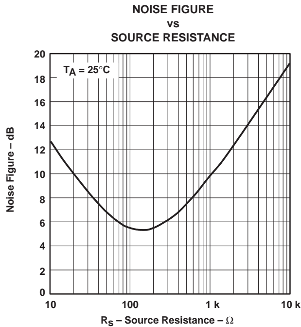
Figure 52. Noise Figure vs Source Resistance
