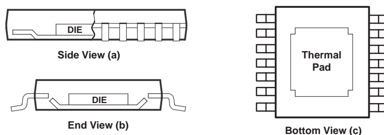
Figure 49. Views of Thermally Enhanced PWP Package
