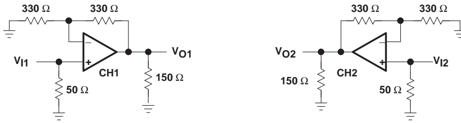
Figure 2. THS6062 Crosstalk Test Circuit
