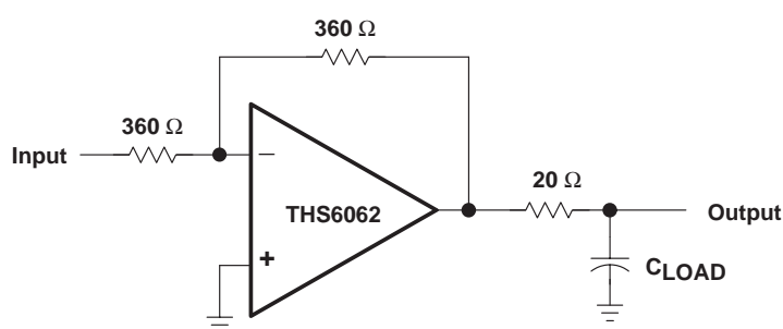
Figure 44. Driving a Capacitive Load
