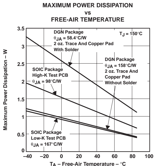
Figure 48. Maximum Power Dissipation vs Free-Air Temperature
