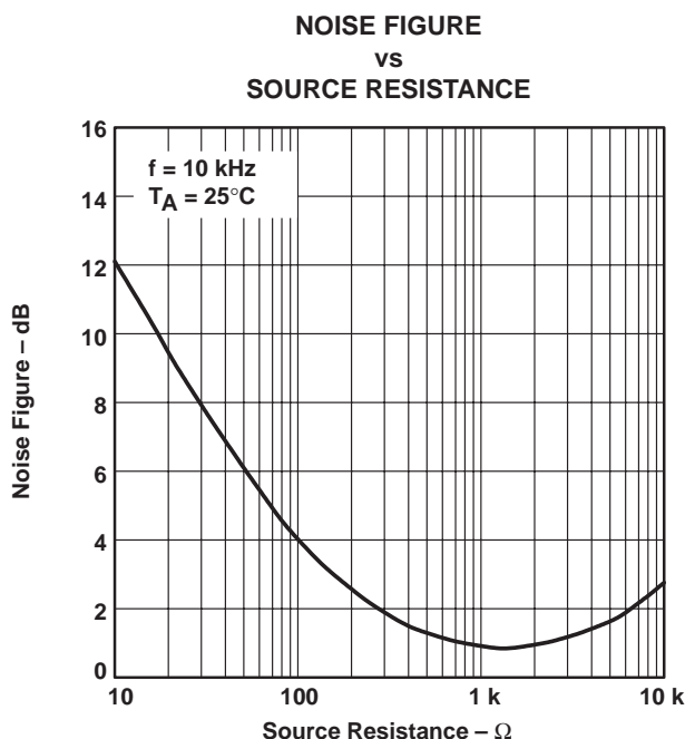
Figure 41. Noise Figure vs Source Resistance
