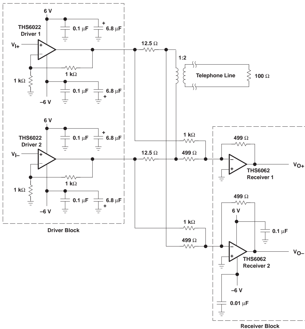
Figure 39. THS6062 Client-Side ADSL Application
