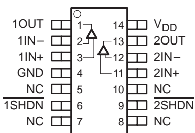
TLC073 D OR N PACKAGE (TOP VIEW)
