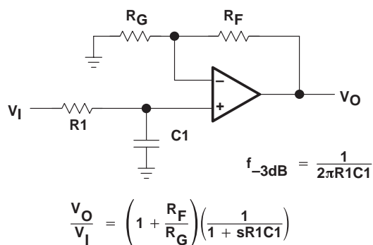
Figure 50. Single-Pole Low-Pass Filter
