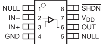
TLC070 D, DGN OR P PACKAGE (TOP VIEW)
