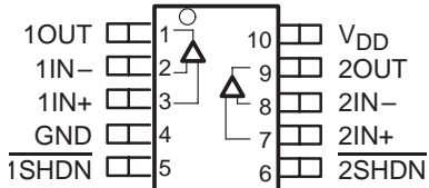
TLC073 DGQ PACKAGE (TOP VIEW)
