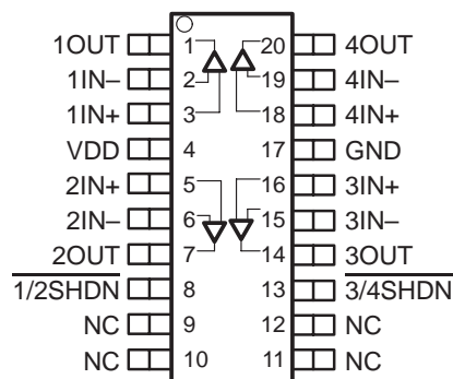
TLC075 PWP PACKAGE (TOP VIEW)
