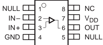
TLC071 D, DGN OR P PACKAGE (TOP VIEW)
