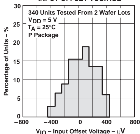
DISTRIBUTION OF TLC27M7 INPUT OFFSET VOLTAGE
