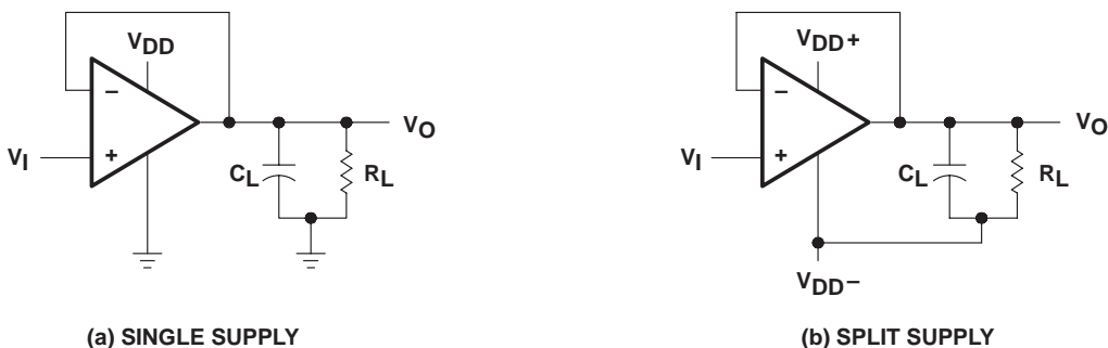
Figure 1. Unity-Gain Amplifier
