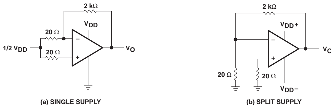
Figure 2. Noise-Test Circuit
