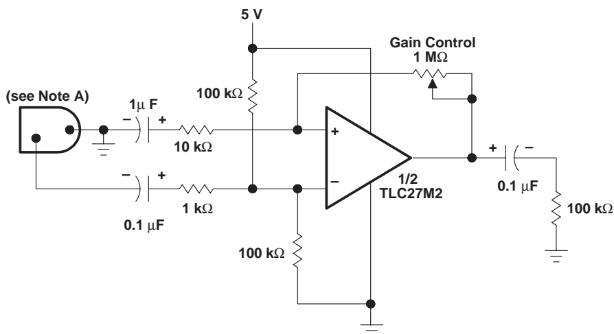
Figure 46. Microphone Preamplifier
