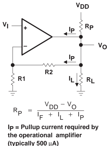
Figure 42. Resistive Pullup to Increase V_{OH}
