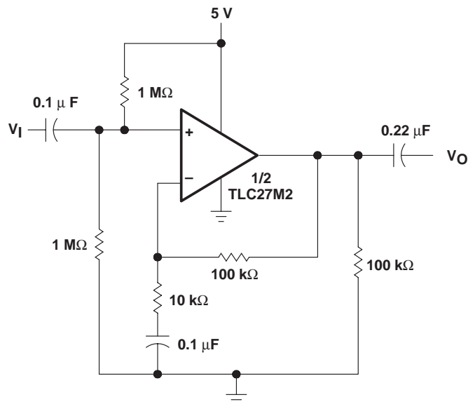
Figure 49. Single-Rail AC Amplifiers
