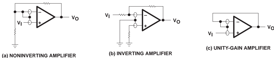
Figure 40. Guard-Ring Schemes
