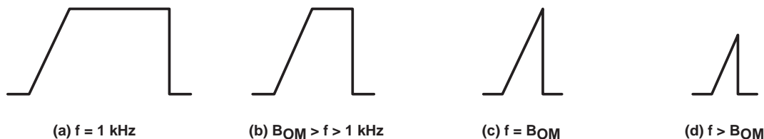
Figure 5. Full-Power-Response Output Signal
