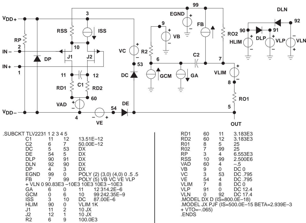
Figure 57. Boyle Macromodel and Subcircuit
