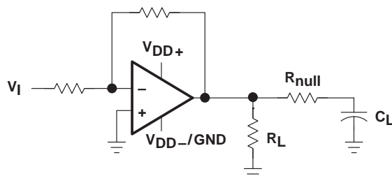
Figure 56. Series-Resistance Circuit
