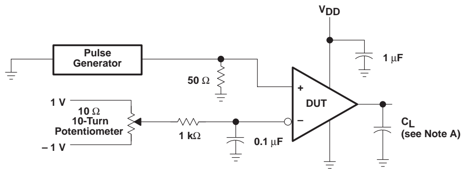
TEST CIRCUIT
