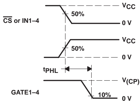
Figure 2. Gate Control Turn-Off
