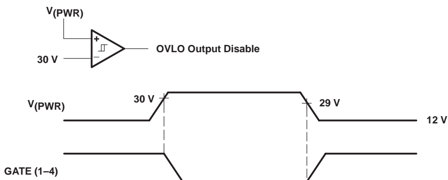
Figure 10. Over-Voltage Lockout Waveform
