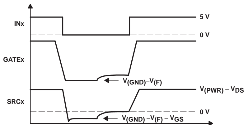
Figure 19. Inductive Load Waveforms
