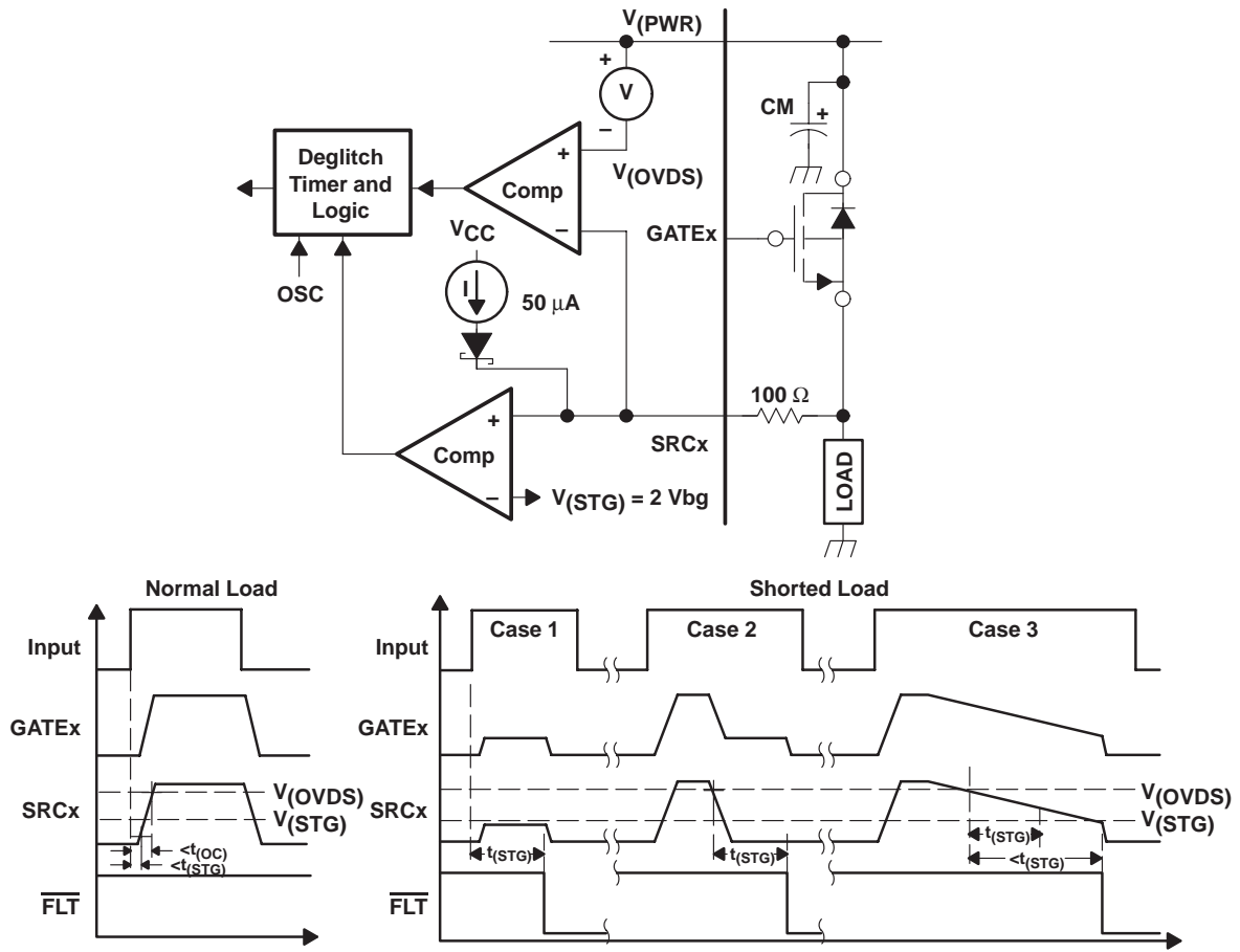
Figure 17. Short-to-Ground Fault Detection
