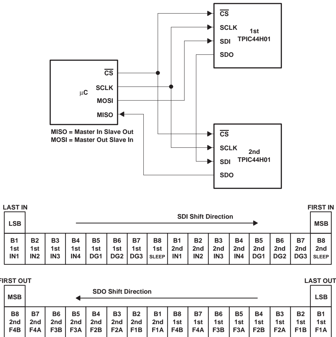
Figure 7. Cascading Multiple TPIC44H01s
