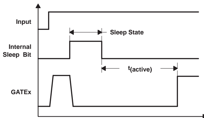
Figure 18. Sleep State Timing Diagram
