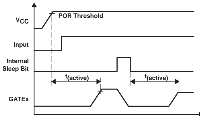
Figure 4. Power-Up Waveforms
