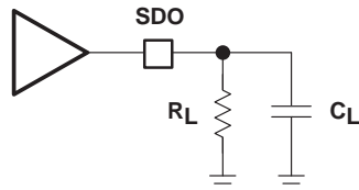
SDO Output Test Schematic
