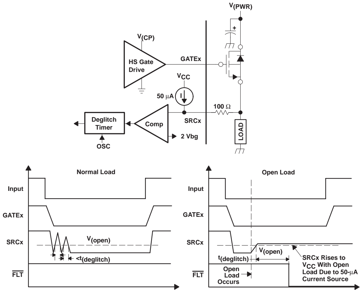
Figure 11. Open-Load Fault Detection
