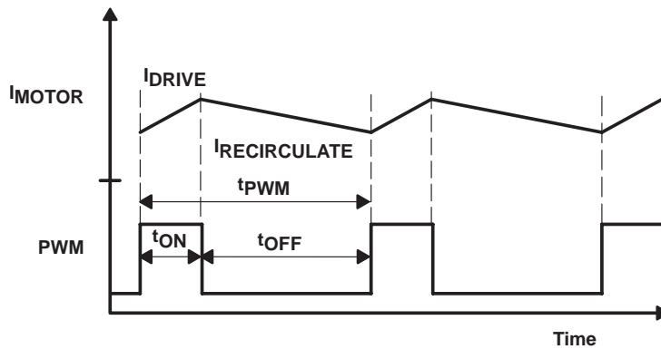
Figure 4. Motor Current Waveform
