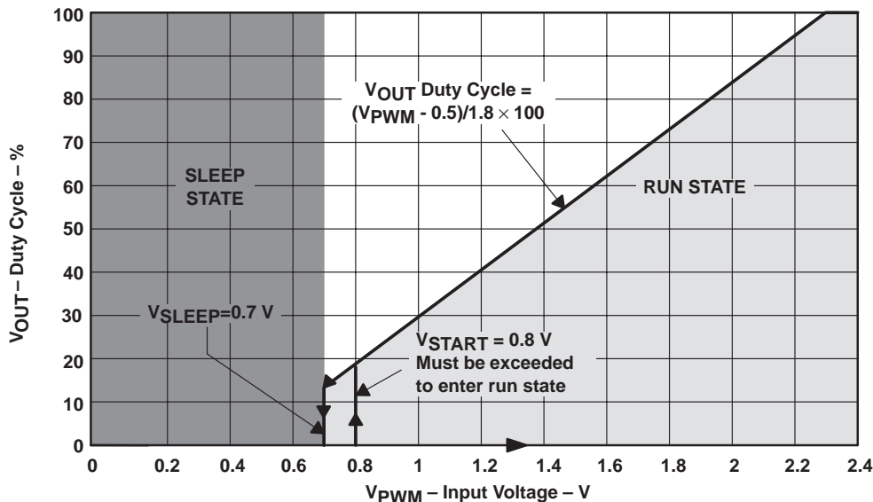
Figure 6. Relationship of V_{O_{UT}} Duty Cycle, V_{S_{TART}} , and V_{S_{LEEP}} vs V_{P_{PWM}} Input Voltage
