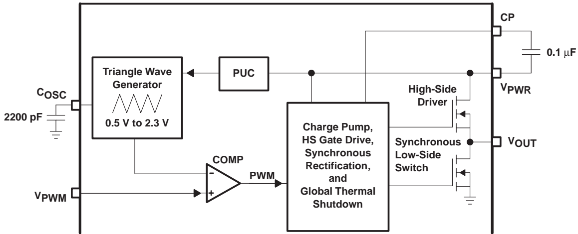
Figure 3. High-Side PWM Drive
