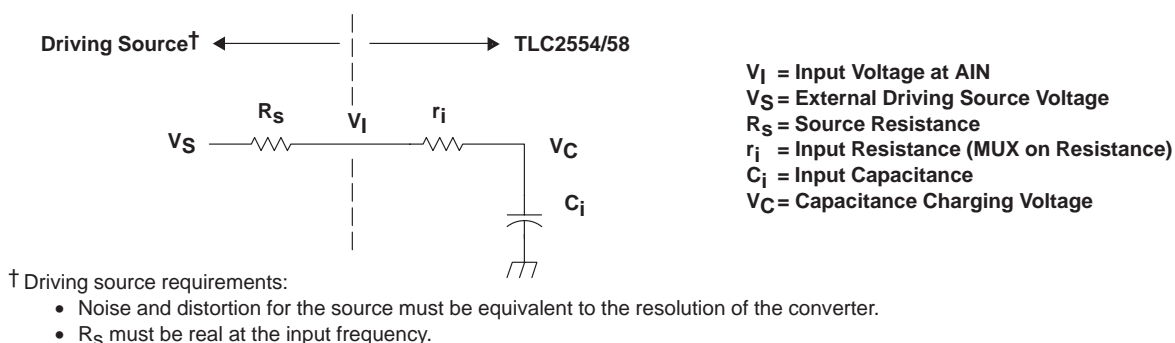
Figure 37. Equivalent Input Circuit Including the Driving Source
