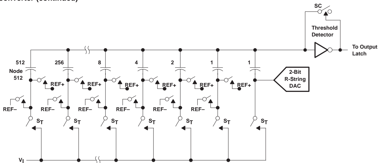
Figure 1. Simplified Model of the Successive-Approximation System
