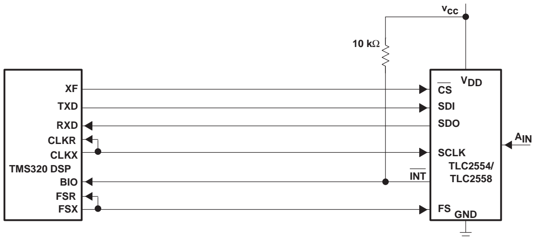
Figure 36. Typical Interface to a TMS320 DSP
