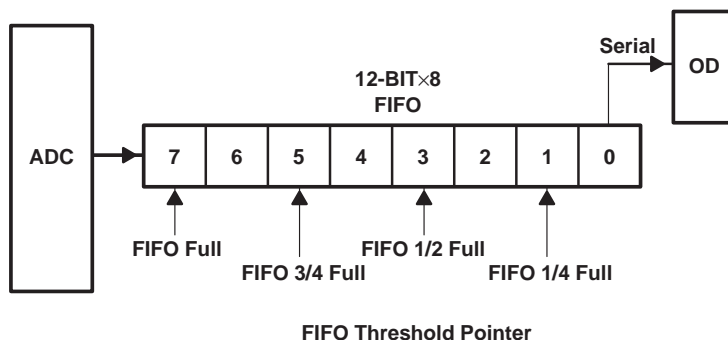
Figure 15. TLC2554/TLC2558 FIFO
