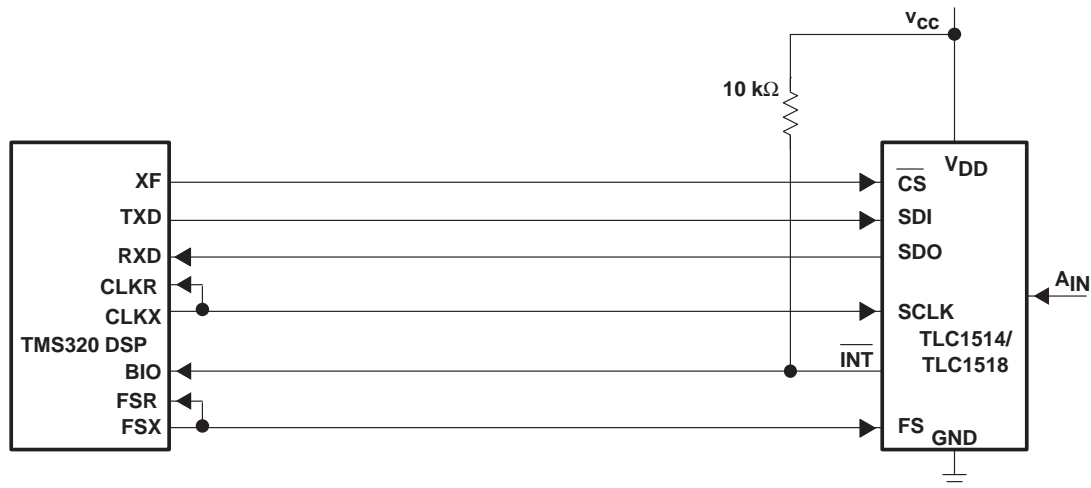
Figure 37. Typical Interface to a TMS320 DSP
