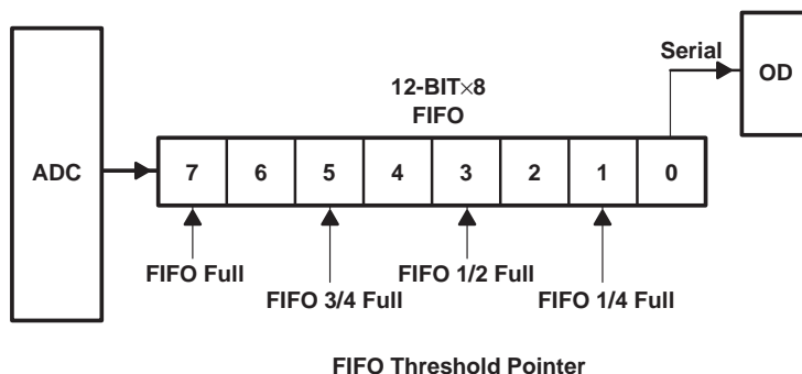
Figure 15. TLC1514/TLC1518 FIFO
