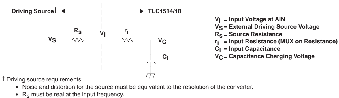
Figure 38. Equivalent Input Circuit Including the Driving Source
