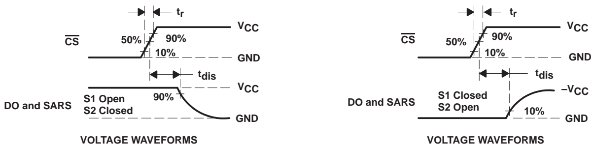
VOLTAGE WAVEFORMS
