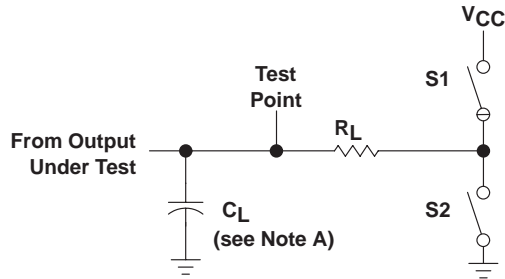
LOAD CIRCUIT
