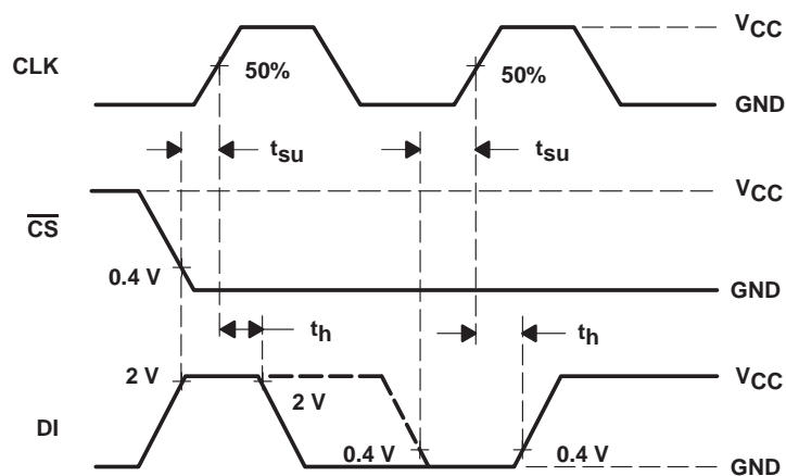
Figure 1. Data-Input Timing
