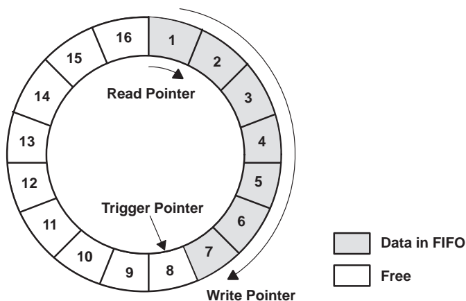
Figure 4. Circular Buffer
