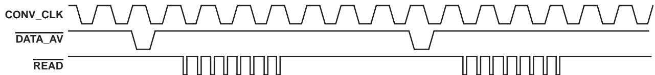
Figure 7. Trigger Level 8 Selected
