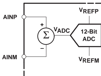
Figure 16. Differential Input Stage
