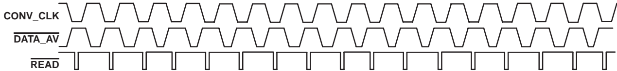
Figure 5. Trigger Level 1 Selected
