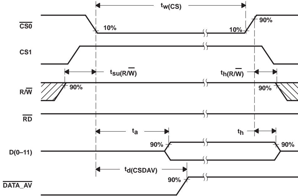
Figure 11. Read Timing Diagram Using \overline{R/W} ( \overline{CS0} -controlled)
