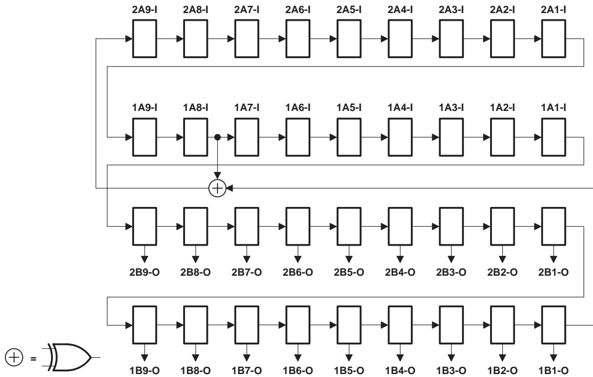
Figure 4. 36-Bit PRPG Configuration ( 1\overline{OEAB} = 2\overline{OEAB} = 0 , 1\overline{OEBA} = 2\overline{OEBA} = 1 )
