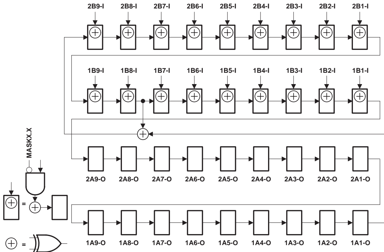
Figure 7. 36-Bit PSA Configuration ( 1\overline{OEAB} = 2\overline{OEAB} = 1 , 1\overline{OEBA} = 2\overline{OEBA} = 0 )
