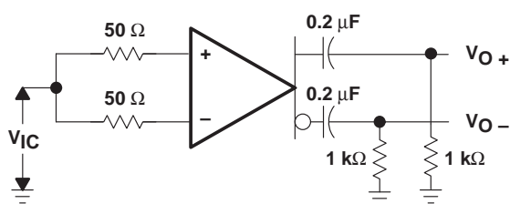
Figure 3. Test Circuit
