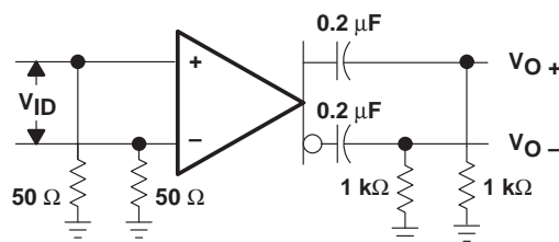
Figure 2. Test Circuit
