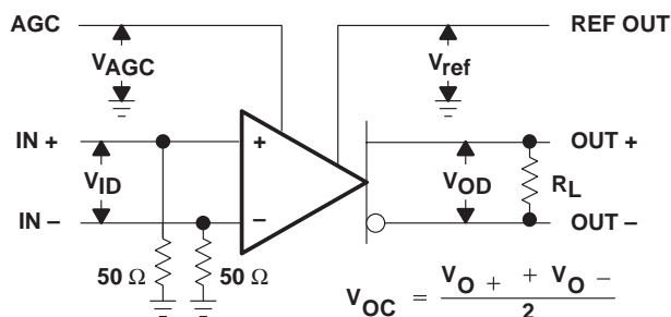
Figure 1. Test Circuit
