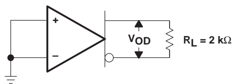
Figure 4. Test Circuit
