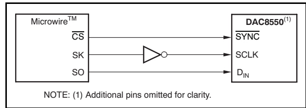
Figure 51. DAC8550 to Microwire Interface
