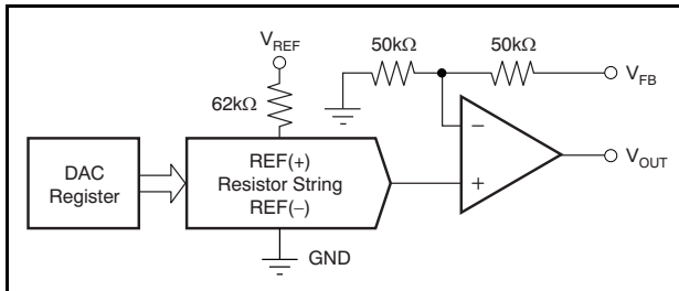
Figure 45. DAC8550 Architecture
