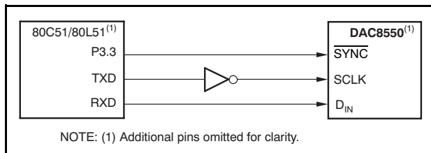
Figure 50. DAC8550 to 80C51/80L51 Interface
