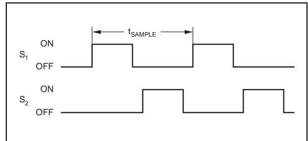
Figure 36. S_1 and S_2 Switch Timing for Figure 37
