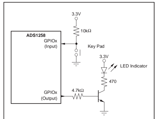
Figure 65. GPIO Connections
