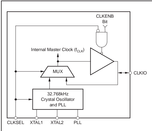
Figure 38. Clock Generation Block Diagram
