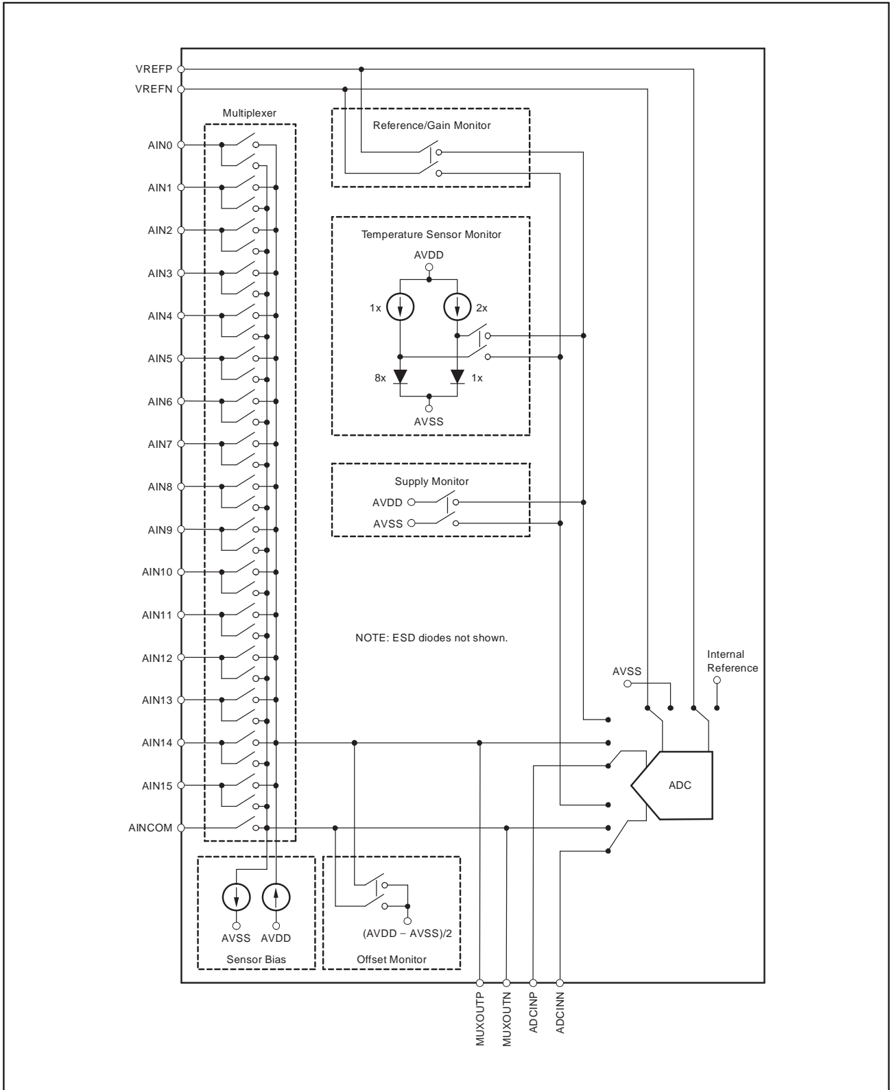
Figure 35. Input Multiplexer
