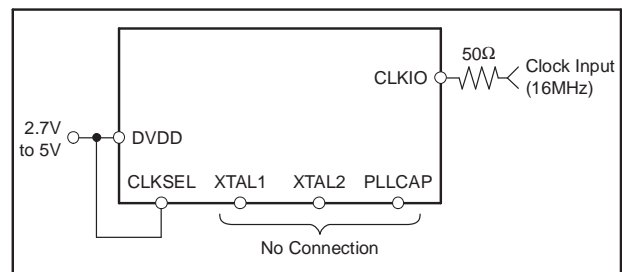
Figure 40. External Clock Connection
