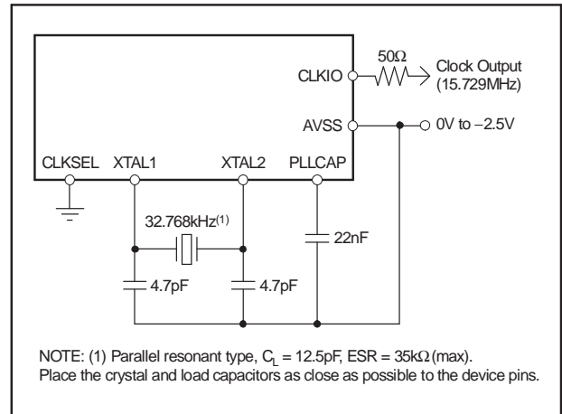
Figure 39. Crystal Oscillator Connection
