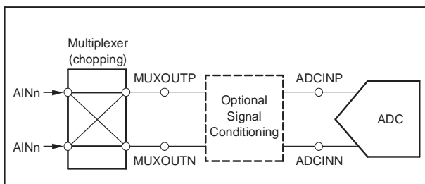
Figure 48. External Chopping
