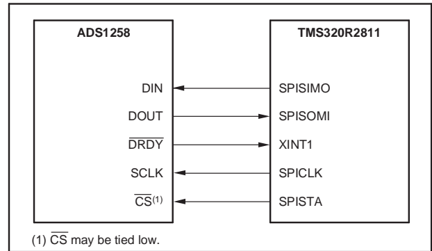
Figure 64. Connection to a TMS320R2811 DSP
