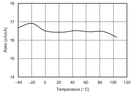
SENSOR BIAS CURRENT SOURCE RATIO vs TEMPERATURE
