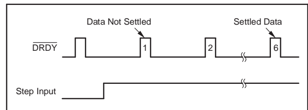
Figure 46. Asynchronous Step-Input Settling Time (Fixed-Channel Mode, DRATE[1:0] = 11)
