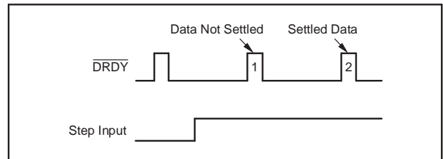
Figure 45. Asynchronous Step-Input Settling Time (DRATE[1:0] = 10, 01, 00)
