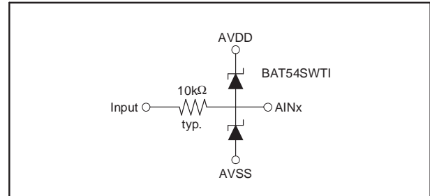
Figure 61. Input Overload Protection
