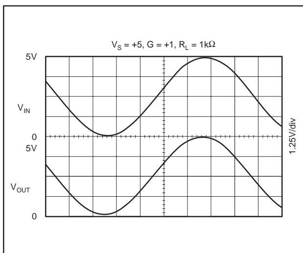
Figure 1. Rail-to-Rail Input and Output
