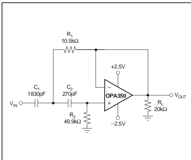
Figure 9. 10kHz High-Pass Filter
