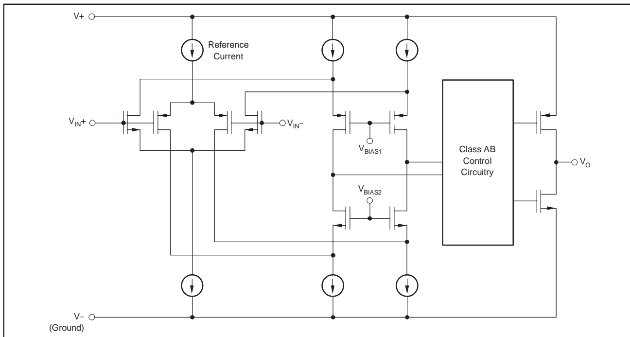
Figure 2. Simplified Schematic
