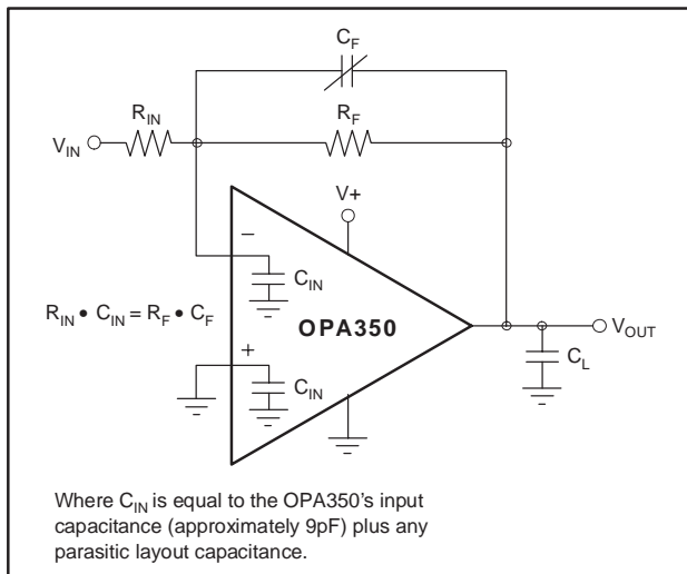
Figure 4. Feedback Capacitor Improves Dynamic Performance
