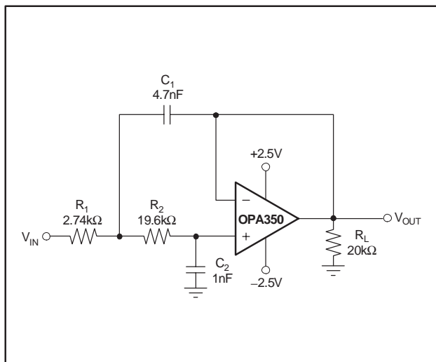
Figure 8. 10kHz Low-Pass Filter
