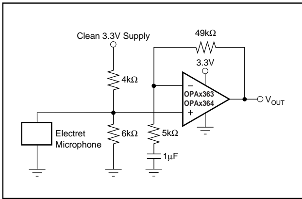
FIGURE 10. Microphone Preamplifier.
