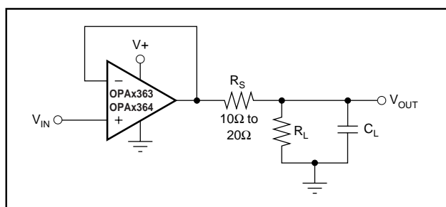
FIGURE 3. Improving Capacitive Load Drive.
