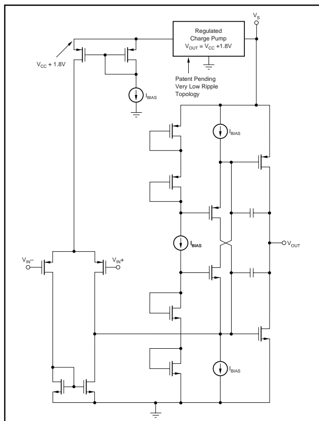
FIGURE 2. Simplified Schematic.
