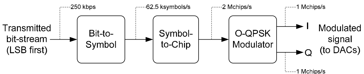
Figure 12: Modulation
