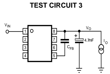
NOISE LEVEL TEST CIRCUIT
