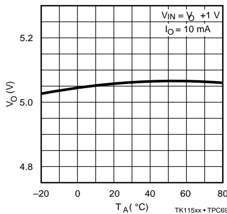
TK11550 OUTPUT VOLTAGE vs TEMPERATURE
