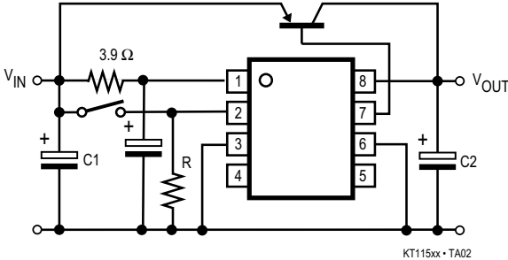
ACTIVE HIGH CONTROL WITH CURRENT BOOST
