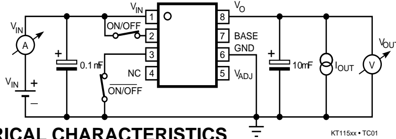
TEST CIRCUIT 1
