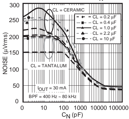
TK71730S NOISE vs. C_N
