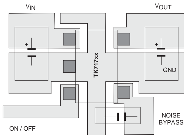
SOT23-5 BOARDLAYOUT
