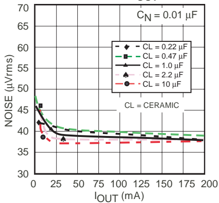
NOISE vs. I_{OUT}
