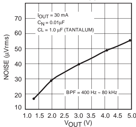
NOISE vs V_{OUT}
