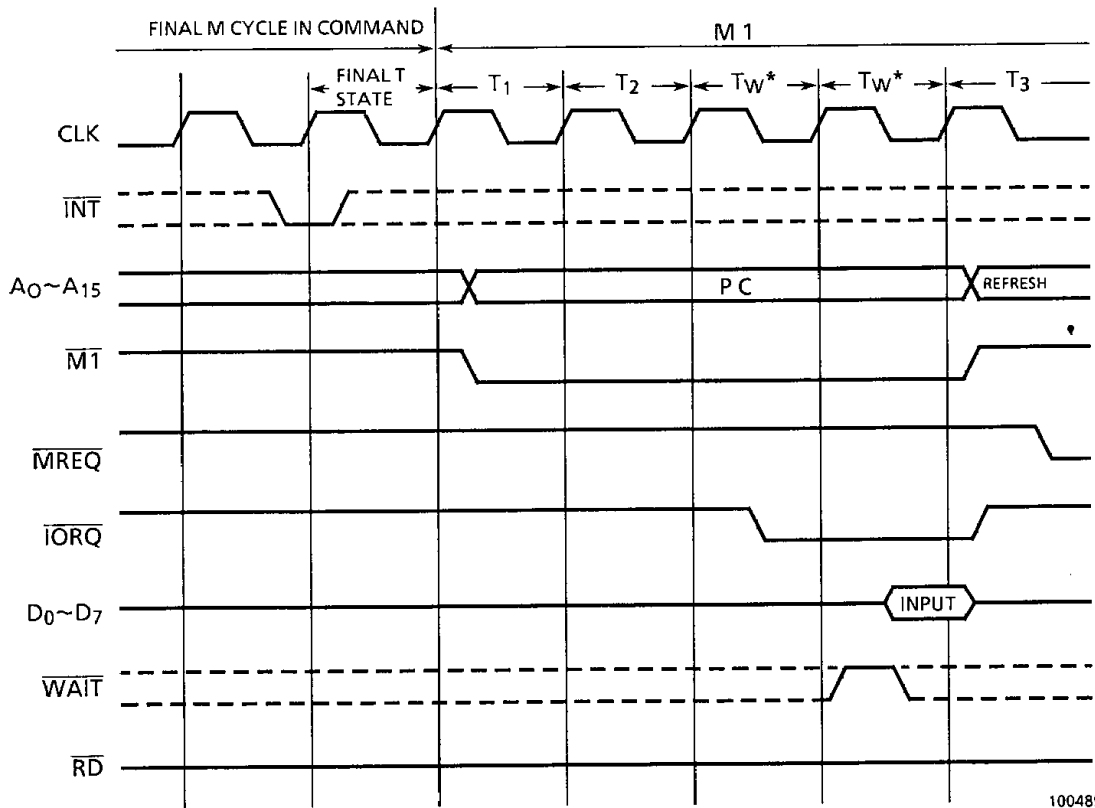
Figure 3.32 Interrupt Acknowledge
