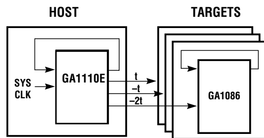
Figure 3. Board-to-Board Synchronization
