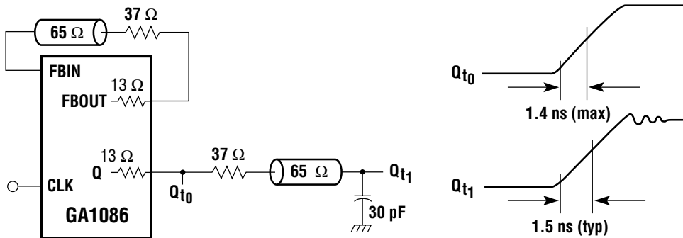
Figure 9. Unbalanced Termination
