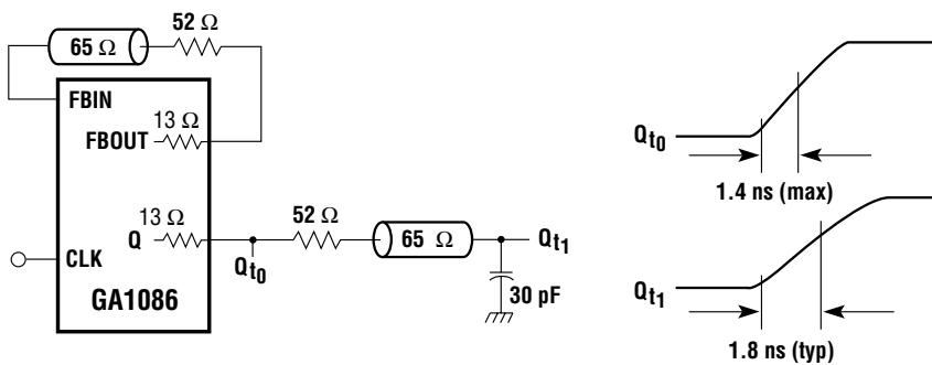
Figure 8. Balanced Termination
