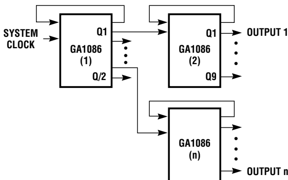
Figure 2. Low-Skew Clock Distribution
