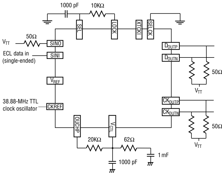
Figure 1. Typical Application
