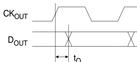
Figure 5. Clock-to-Data Timing
