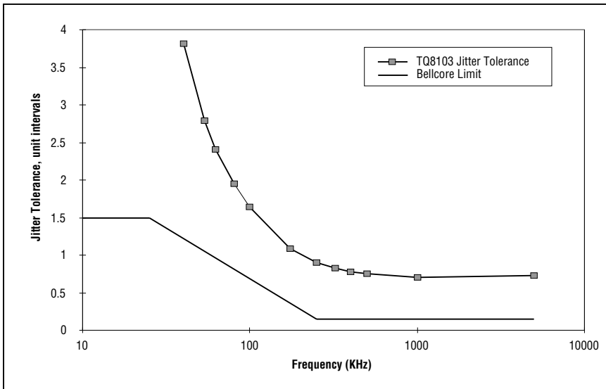
Figure 6. Jitter Tolerance
