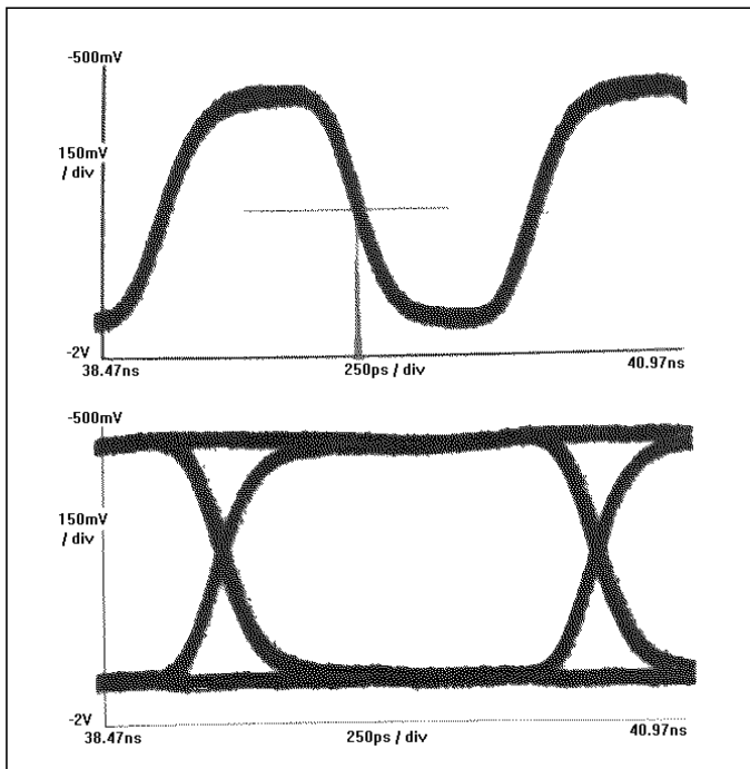
Figure 7. Output Eye Diagram with extracted clock
