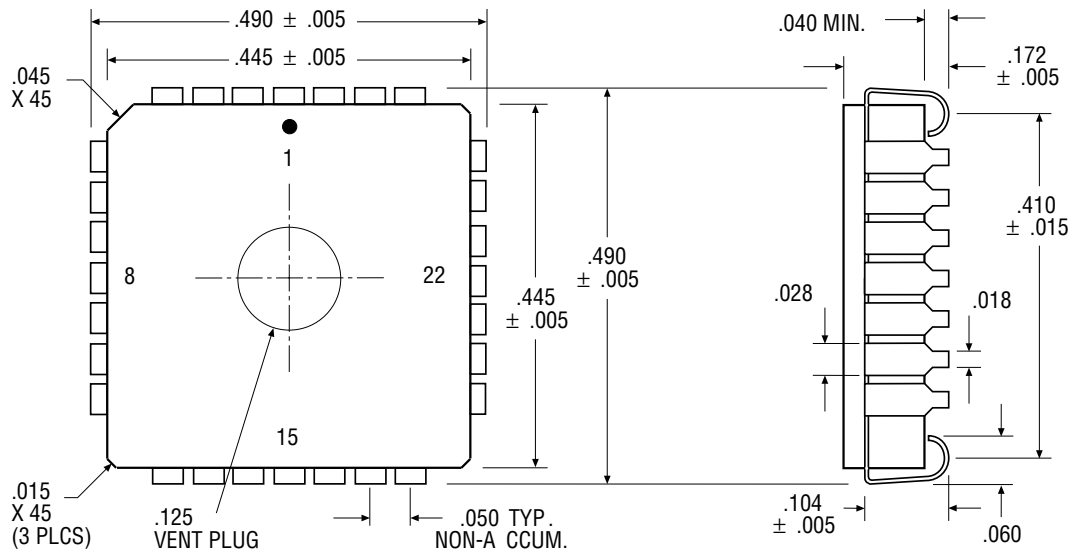
Figure 8. TQ8103 Package Dimensions
