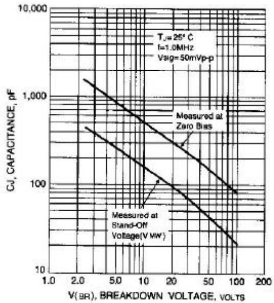
Fig. 4-TYPICAL JUNCTION CAPACITANCE
