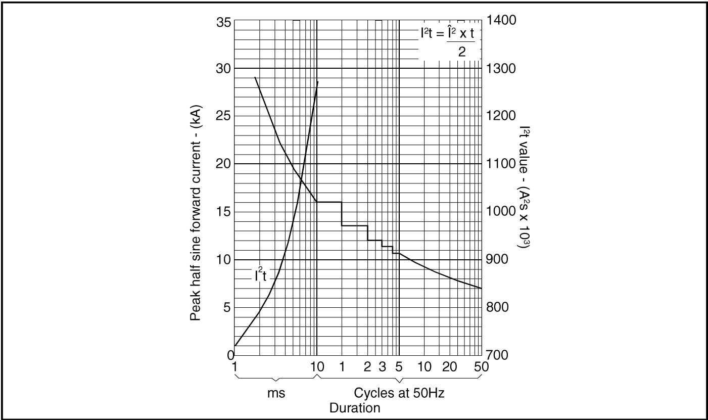
Fig. 5 Surge (non-repetitive) forward current vs time (with 50% V_{RRM} , T_{case} = 175C )
