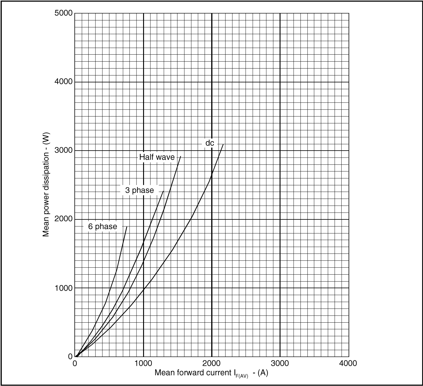
Fig. 2 Dissipation curves
