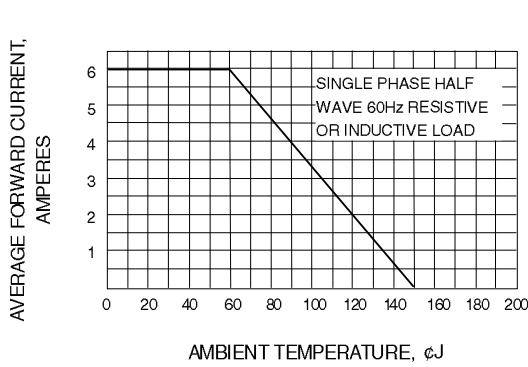
Fig. 2-FORWARD DERATING CURVE
