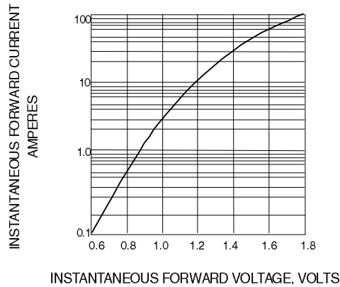
Fig. 4-TYPICAL FORWARD CHARACTERISTIC
