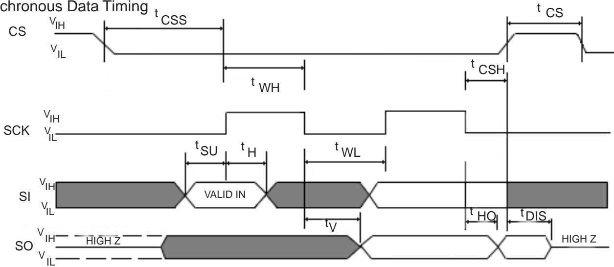
WREN Timing
