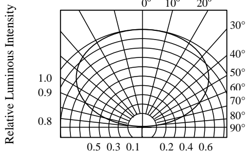
FIG.6 RADIATION DIAGRAM
